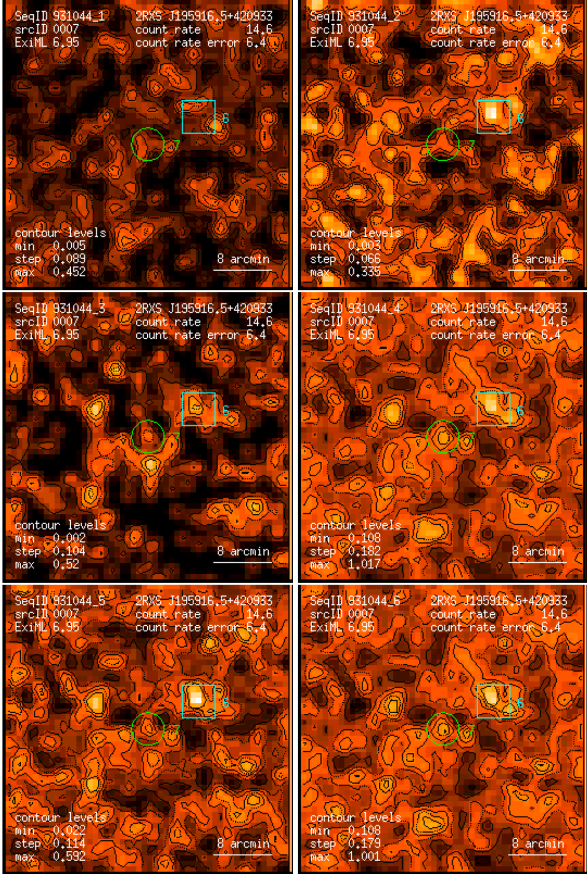
Figure 7: RASS 931044: detection 0007: band rate images, Gaussian filter: (1) PSPC channels 11 – 41, (2) 52 – 90, (3) 91 – 201, (4) 11 – 235, (5) 52 – 201, (6) 11 – 201. Broad band rates in counts/ks. Band rate contour levels in counts/ks/arcmin 2 .
