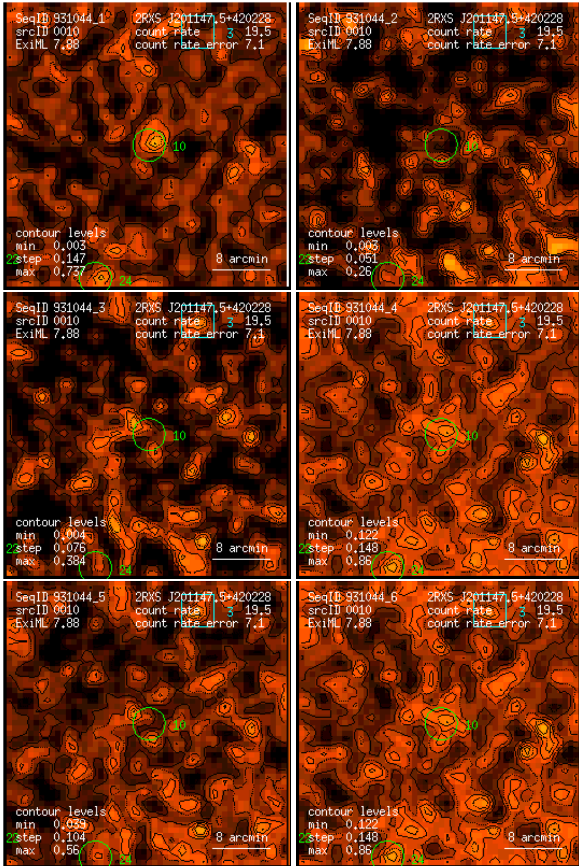
Figure 10: RASS 931044: detection 0010: band rate images, Gaussian filter: (1) PSPC channels 11 – 41, (2) 52 – 90, (3) 91 – 201, (4) 11 – 235, (5) 52 – 201, (6) 11 – 201. Broad band rates in counts/ks. Band rate contour levels in counts/ks/arcmin 2 .
