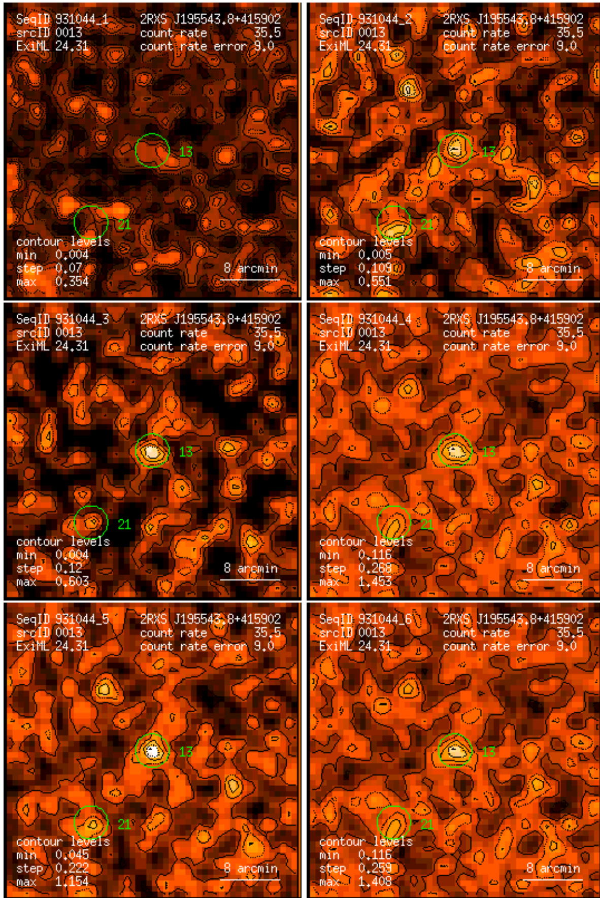
Figure 13: RASS 931044: detection 0013: band rate images, Gaussian filter: (1) PSPC channels 11 – 41, (2) 52 – 90, (3) 91 – 201, (4) 11 – 235, (5) 52 – 201, (6) 11 – 201. Broad band rates in counts/ks. Band rate contour levels in counts/ks/arcmin 2 .
