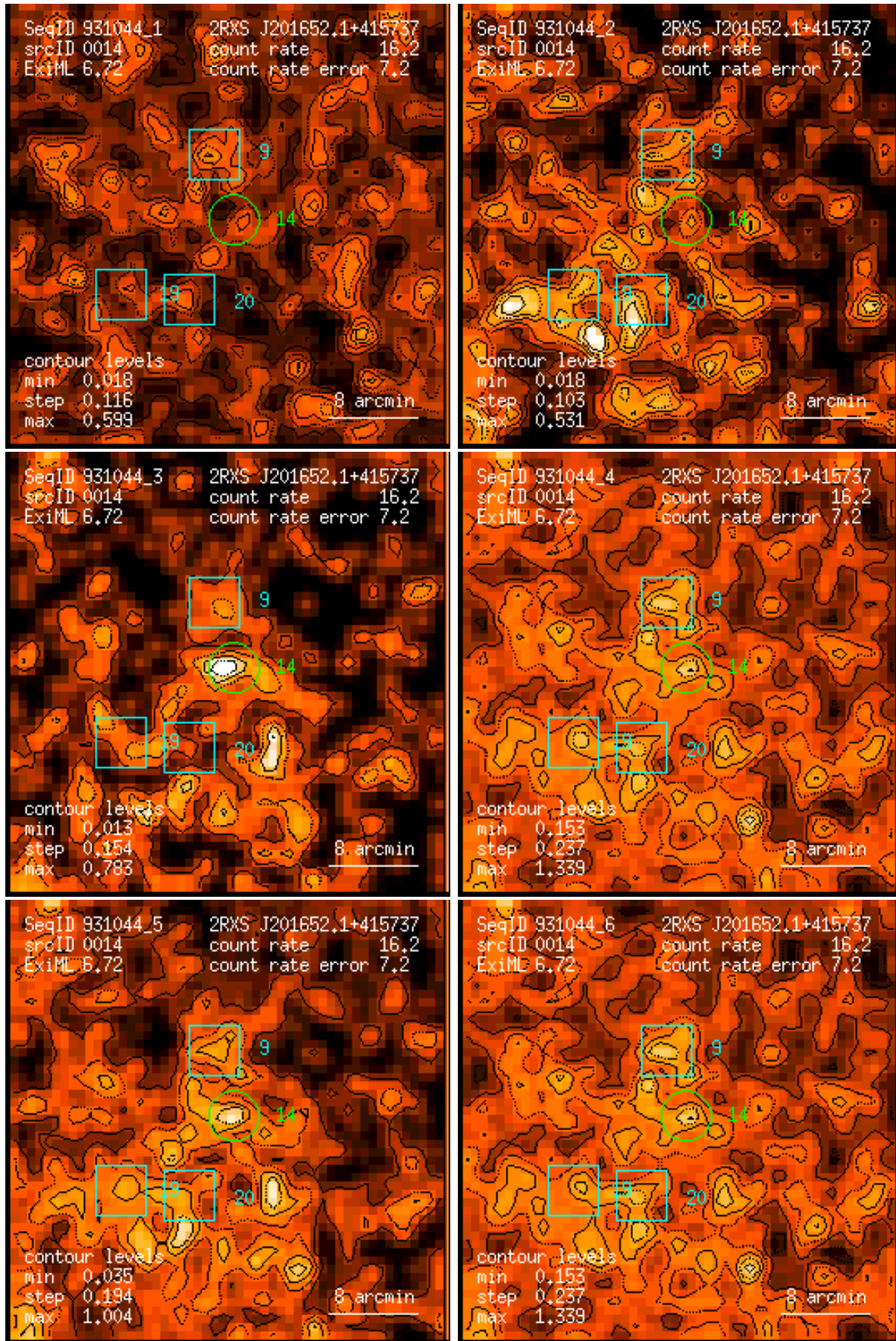
Figure 14: RASS 931044: detection 0014: band rate images, Gaussian filter: (1) PSPC channels 11 – 41, (2) 52 – 90, (3) 91 – 201, (4) 11 – 235, (5) 52 – 201, (6) 11 – 201. Broad band rates in counts/ks. Band rate contour levels in counts/ks/arcmin 2 .
