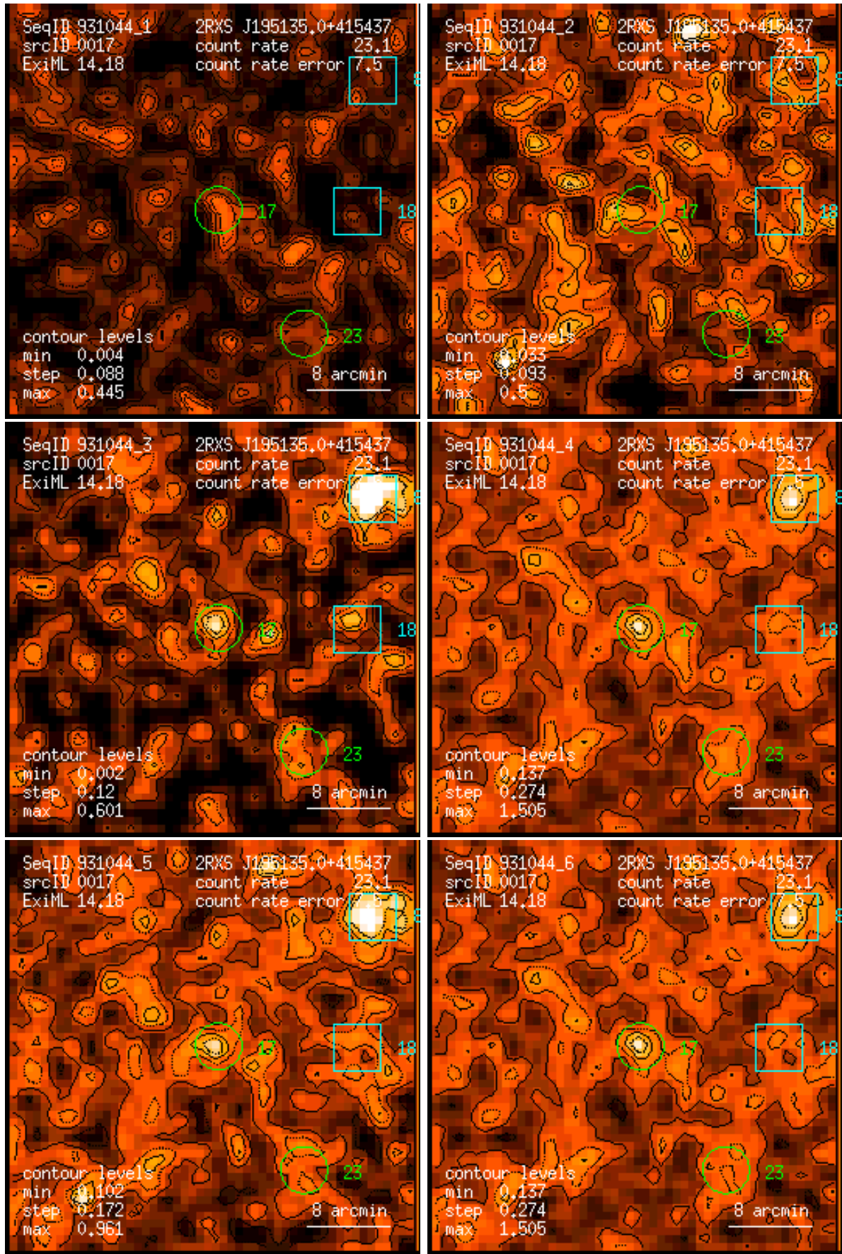
Figure 17: RASS 931044: detection 0017: band rate images, Gaussian filter: (1) PSPC channels 11 – 41, (2) 52 – 90, (3) 91 – 201, (4) 11 – 235, (5) 52 – 201, (6) 11 – 201. Broad band rates in counts/ks. Band rate contour levels in counts/ks/arcmin 2 .
