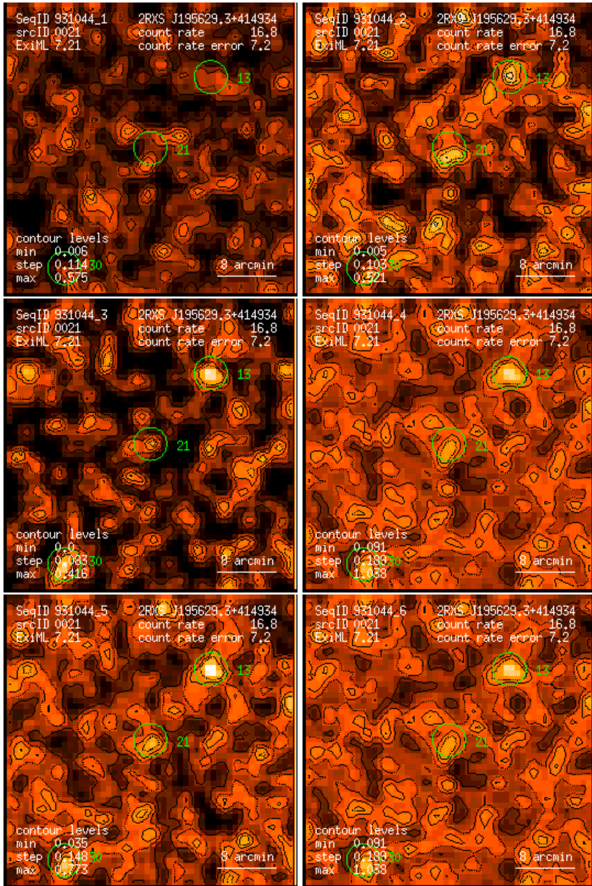
Figure 21: RASS 931044: detection 0021: band rate images, Gaussian filter: (1) PSPC channels 11 – 41, (2) 52 – 90, (3) 91 – 201, (4) 11 – 235, (5) 52 – 201, (6) 11 – 201. Broad band rates in counts/ks. Band rate contour levels in counts/ks/arcmin 2 .
