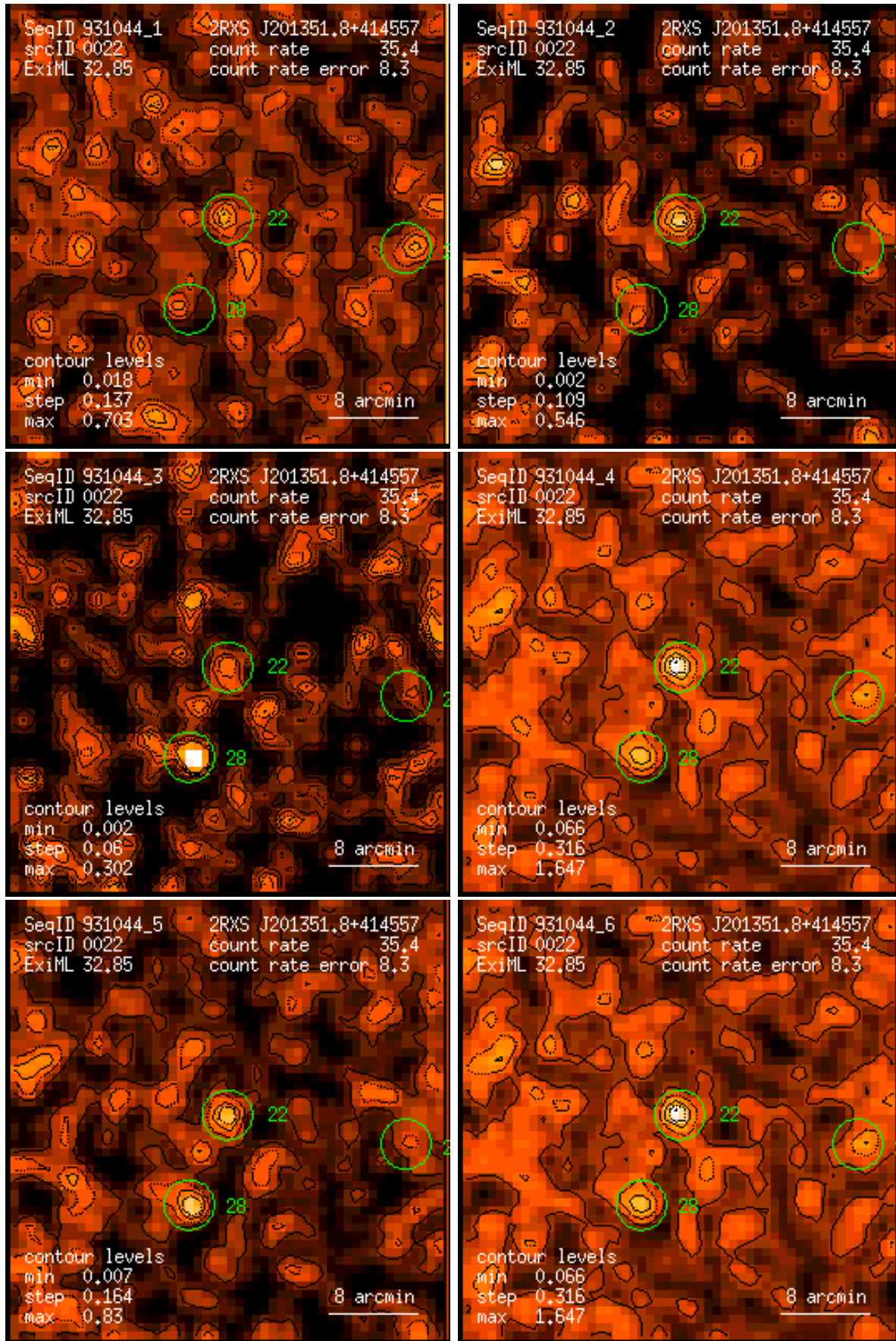
Figure 22: RASS 931044: detection 0022: band rate images, Gaussian filter: (1) PSPC channels 11 – 41, (2) 52 – 90, (3) 91 – 201, (4) 11 – 235, (5) 52 – 201, (6) 11 – 201. Broad band rates in counts/ks. Band rate contour levels in counts/ks/arcmin 2 .
