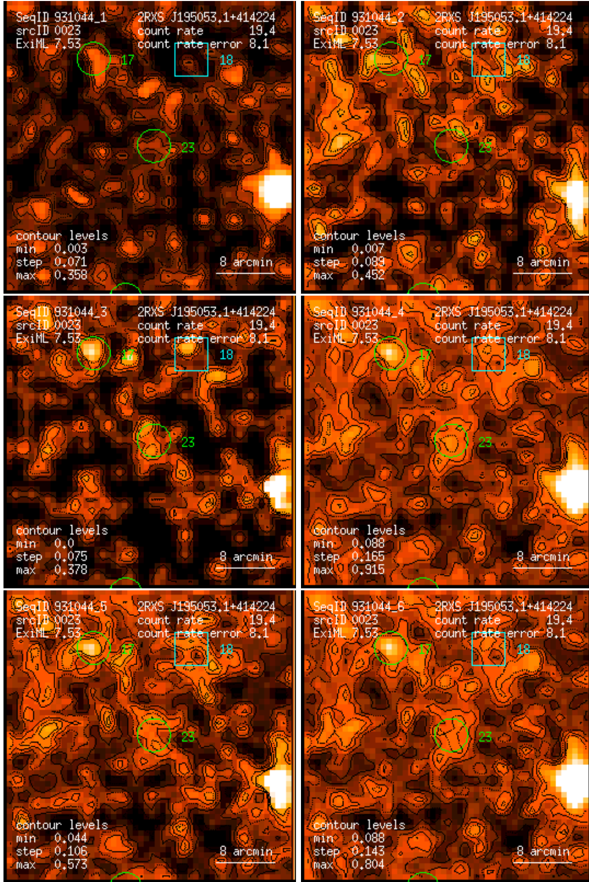
Figure 23: RASS 931044: detection 0023: band rate images, Gaussian filter: (1) PSPC channels 11 – 41, (2) 52 – 90, (3) 91 – 201, (4) 11 – 235, (5) 52 – 201, (6) 11 – 201. Broad band rates in counts/ks. Band rate contour levels in counts/ks/arcmin 2 .
