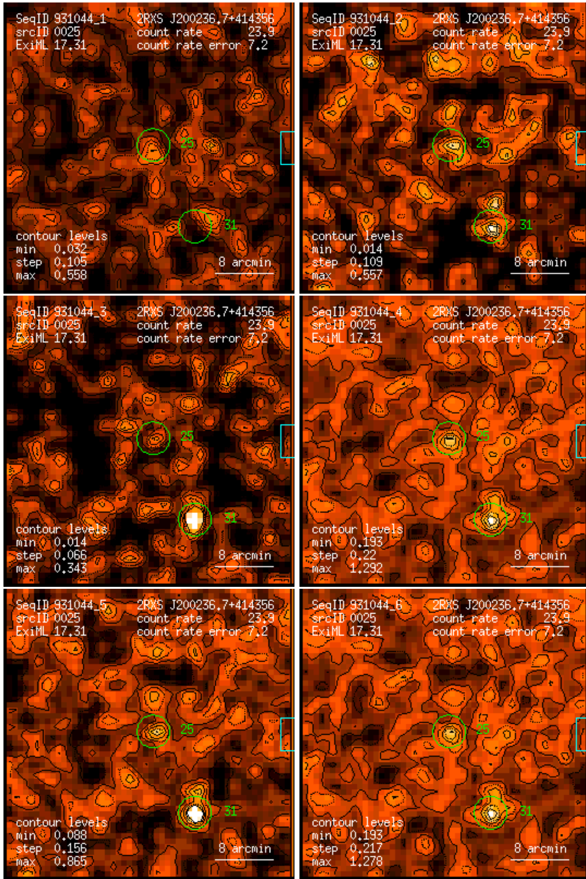
Figure 25: RASS 931044: detection 0025: band rate images, Gaussian filter: (1) PSPC channels 11 – 41, (2) 52 – 90, (3) 91 – 201, (4) 11 – 235, (5) 52 – 201, (6) 11 – 201. Broad band rates in counts/ks. Band rate contour levels in counts/ks/arcmin 2 .
