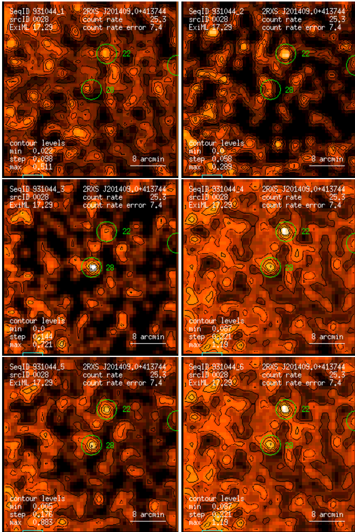
Figure 28: RASS 931044: detection 0028: band rate images, Gaussian filter: (1) PSPC channels 11 – 41, (2) 52 – 90, (3) 91 – 201, (4) 11 – 235, (5) 52 – 201, (6) 11 – 201. Broad band rates in counts/ks. Band rate contour levels in counts/ks/arcmin 2 .
