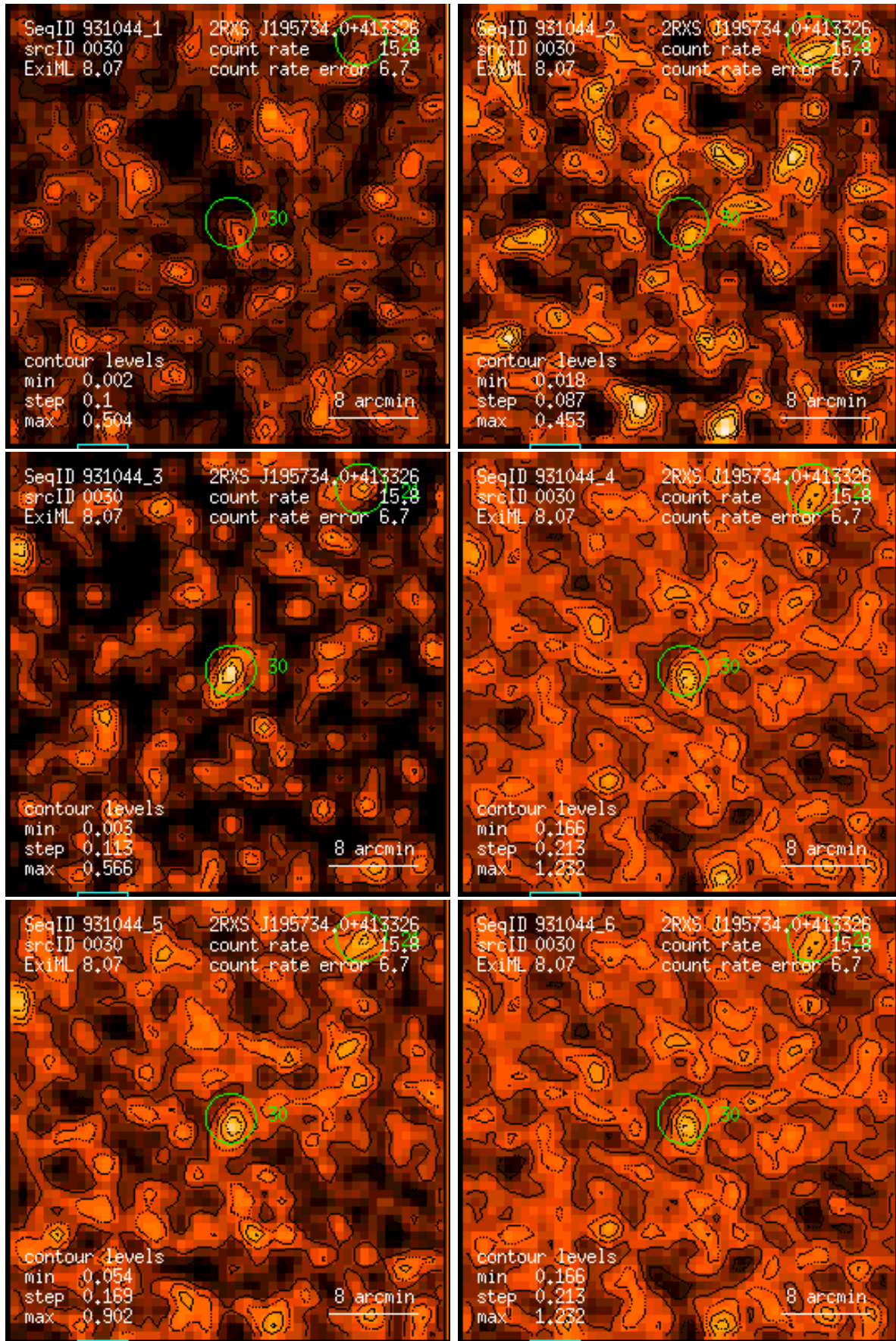
Figure 30: RASS 931044: detection 0030: band rate images, Gaussian filter: (1) PSPC channels 11 – 41, (2) 52 – 90, (3) 91 – 201, (4) 11 – 235, (5) 52 – 201, (6) 11 – 201. Broad band rates in counts/ks. Band rate contour levels in counts/ks/arcmin 2 .
