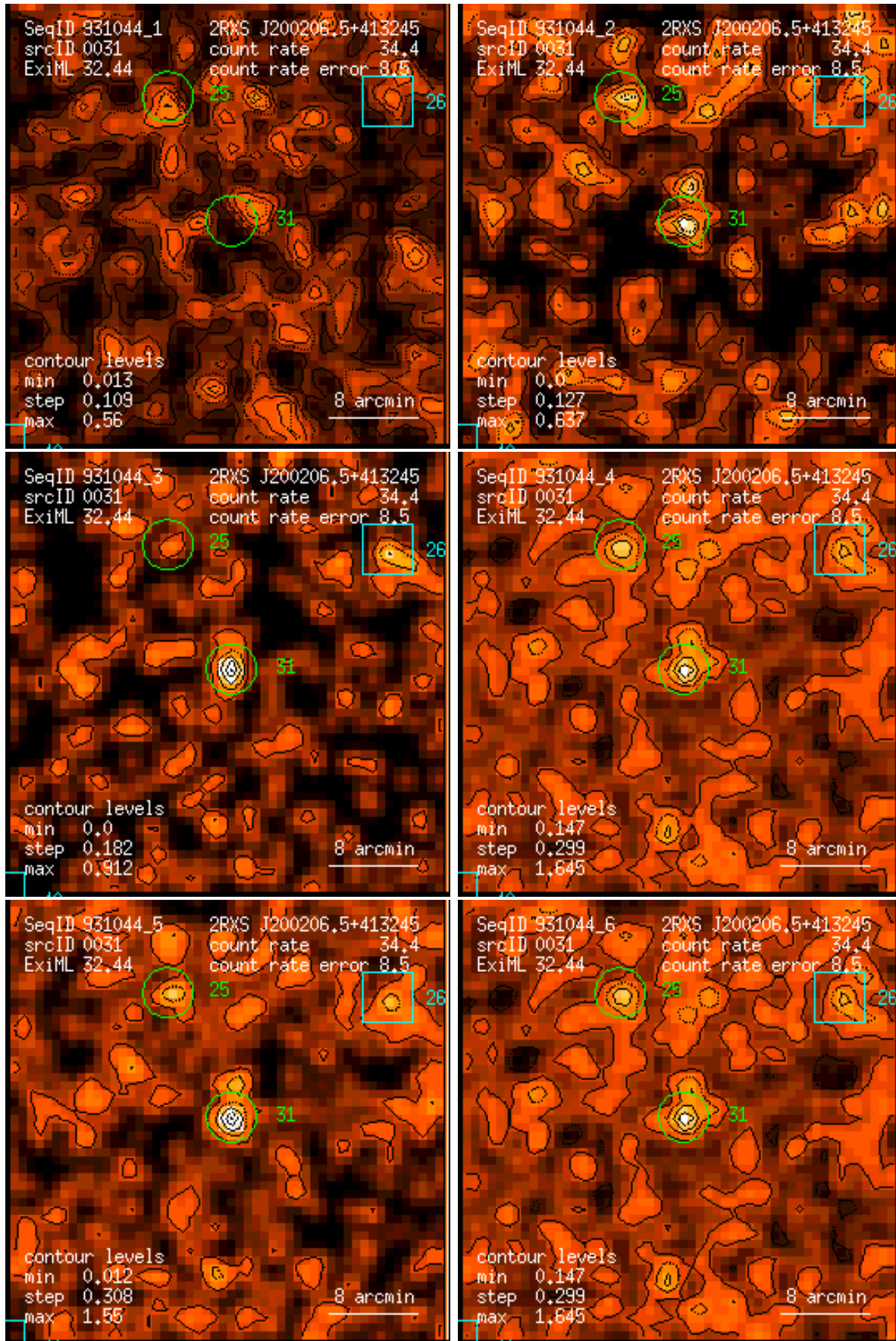
Figure 31: RASS 931044: detection 0031: band rate images, Gaussian filter: (1) PSPC channels 11 – 41, (2) 52 – 90, (3) 91 – 201, (4) 11 – 235, (5) 52 – 201, (6) 11 – 201. Broad band rates in counts/ks. Band rate contour levels in counts/ks/arcmin 2 .
