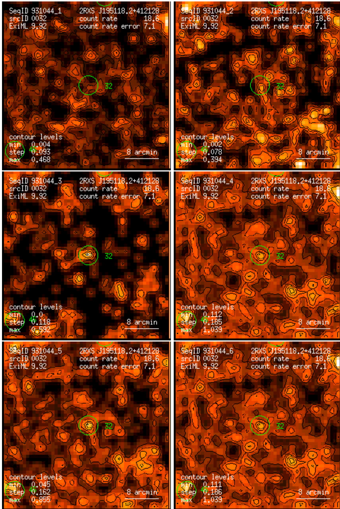
Figure 32: RASS 931044: detection 0032: band rate images, Gaussian filter: (1) PSPC channels 11 – 41, (2) 52 – 90, (3) 91 – 201, (4) 11 – 235, (5) 52 – 201, (6) 11 – 201. Broad band rates in counts/ks. Band rate contour levels in counts/ks/arcmin 2 .
