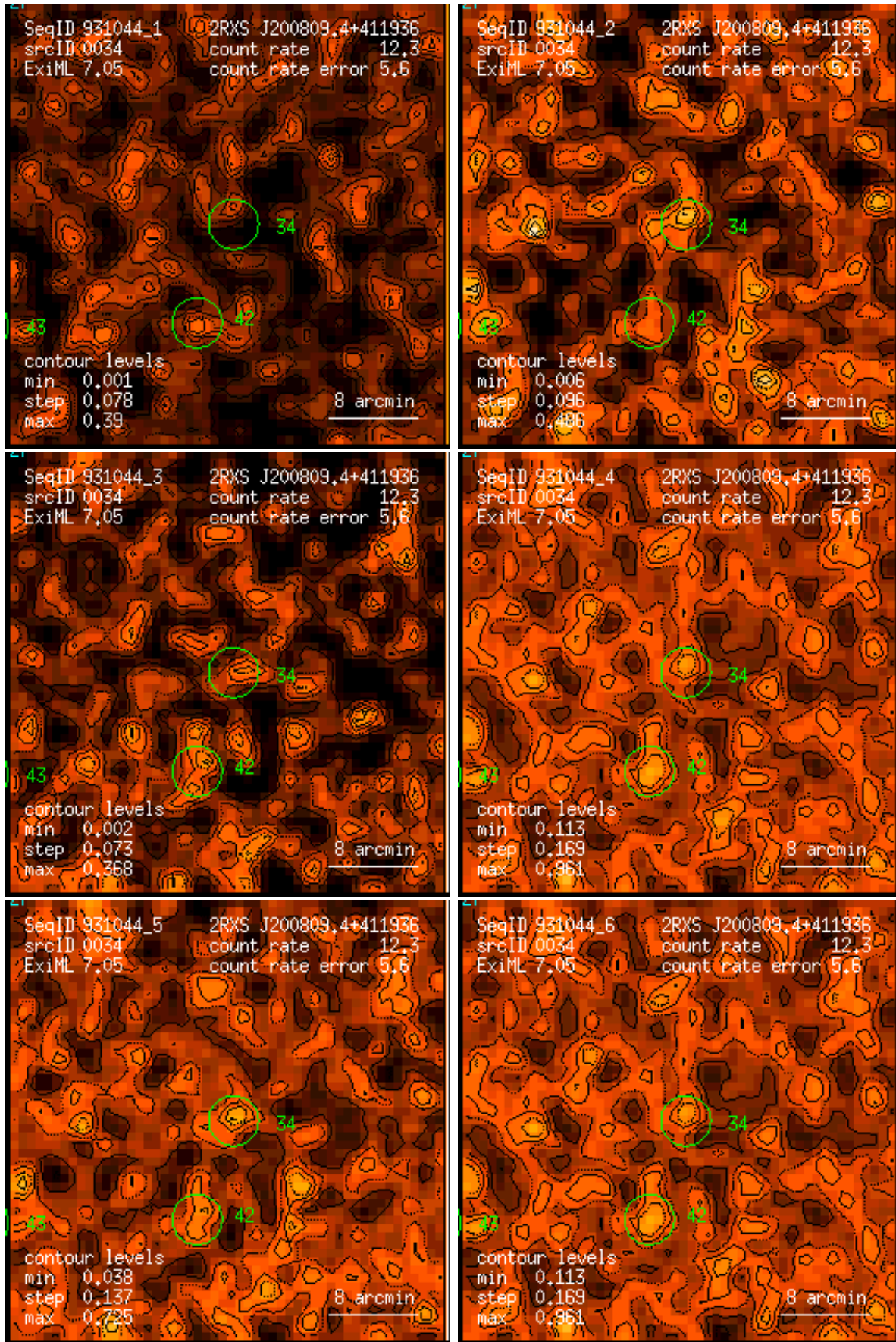
Figure 34: RASS 931044: detection 0034: band rate images, Gaussian filter: (1) PSPC channels 11 – 41, (2) 52 – 90, (3) 91 – 201, (4) 11 – 235, (5) 52 – 201, (6) 11 – 201. Broad band rates in counts/ks. Band rate contour levels in counts/ks/arcmin 2 .
