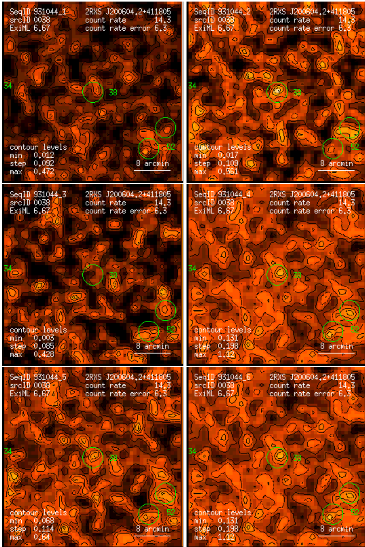
Figure 38: RASS 931044: detection 0038: band rate images, Gaussian filter: (1) PSPC channels 11 – 41, (2) 52 – 90, (3) 91 – 201, (4) 11 – 235, (5) 52 – 201, (6) 11 – 201. Broad band rates in counts/ks. Band rate contour levels in counts/ks/arcmin 2 .
