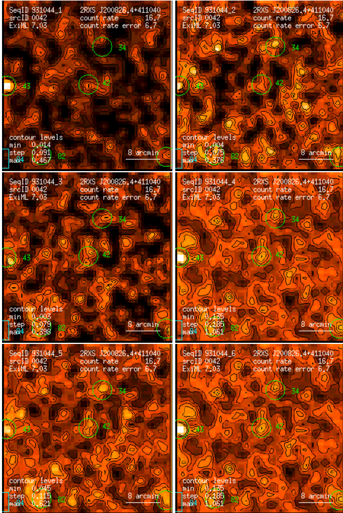
Figure 42: RASS 931044: detection 0042: band rate images, Gaussian filter: (1) PSPC channels 11 – 41, (2) 52 – 90, (3) 91 – 201, (4) 11 – 235, (5) 52 – 201, (6) 11 – 201. Broad band rates in counts/ks. Band rate contour levels in counts/ks/arcmin 2 .
