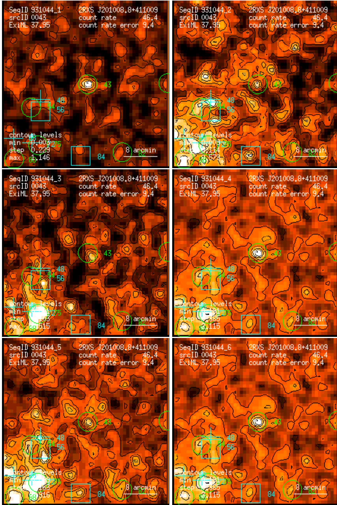
Figure 43: RASS 931044: detection 0043: band rate images, Gaussian filter: (1) PSPC channels 11 – 41, (2) 52 – 90, (3) 91 – 201, (4) 11 – 235, (5) 52 – 201, (6) 11 – 201. Broad band rates in counts/ks. Band rate contour levels in counts/ks/arcmin 2 .
