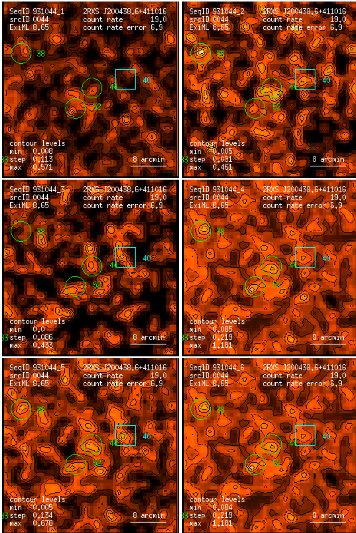
Figure 44: RASS 931044: detection 0044: band rate images, Gaussian filter: (1) PSPC channels 11 – 41, (2) 52 – 90, (3) 91 – 201, (4) 11 – 235, (5) 52 – 201, (6) 11 – 201. Broad band rates in counts/ks. Band rate contour levels in counts/ks/arcmin 2 .
