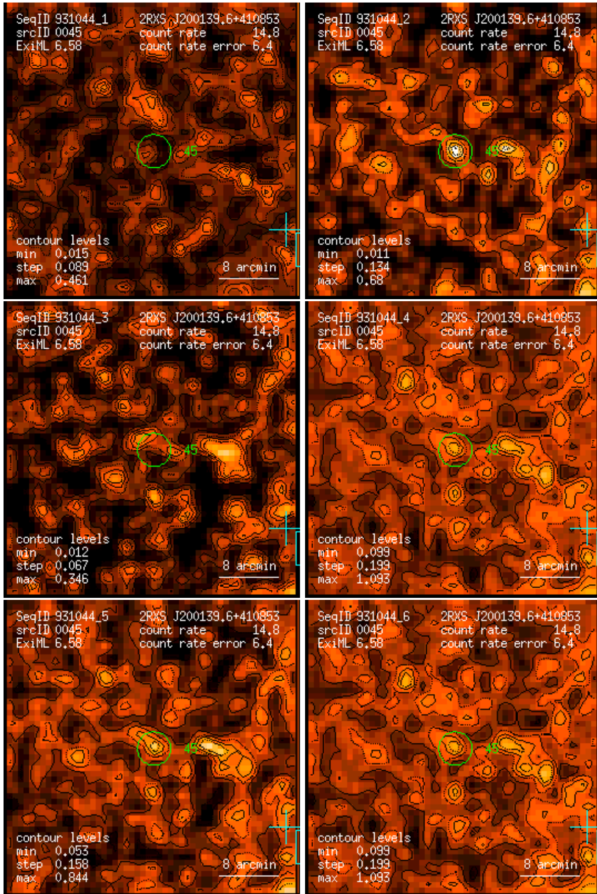
Figure 45: RASS 931044: detection 0045: band rate images, Gaussian filter: (1) PSPC channels 11 – 41, (2) 52 – 90, (3) 91 – 201, (4) 11 – 235, (5) 52 – 201, (6) 11 – 201. Broad band rates in counts/ks. Band rate contour levels in counts/ks/arcmin 2 .
