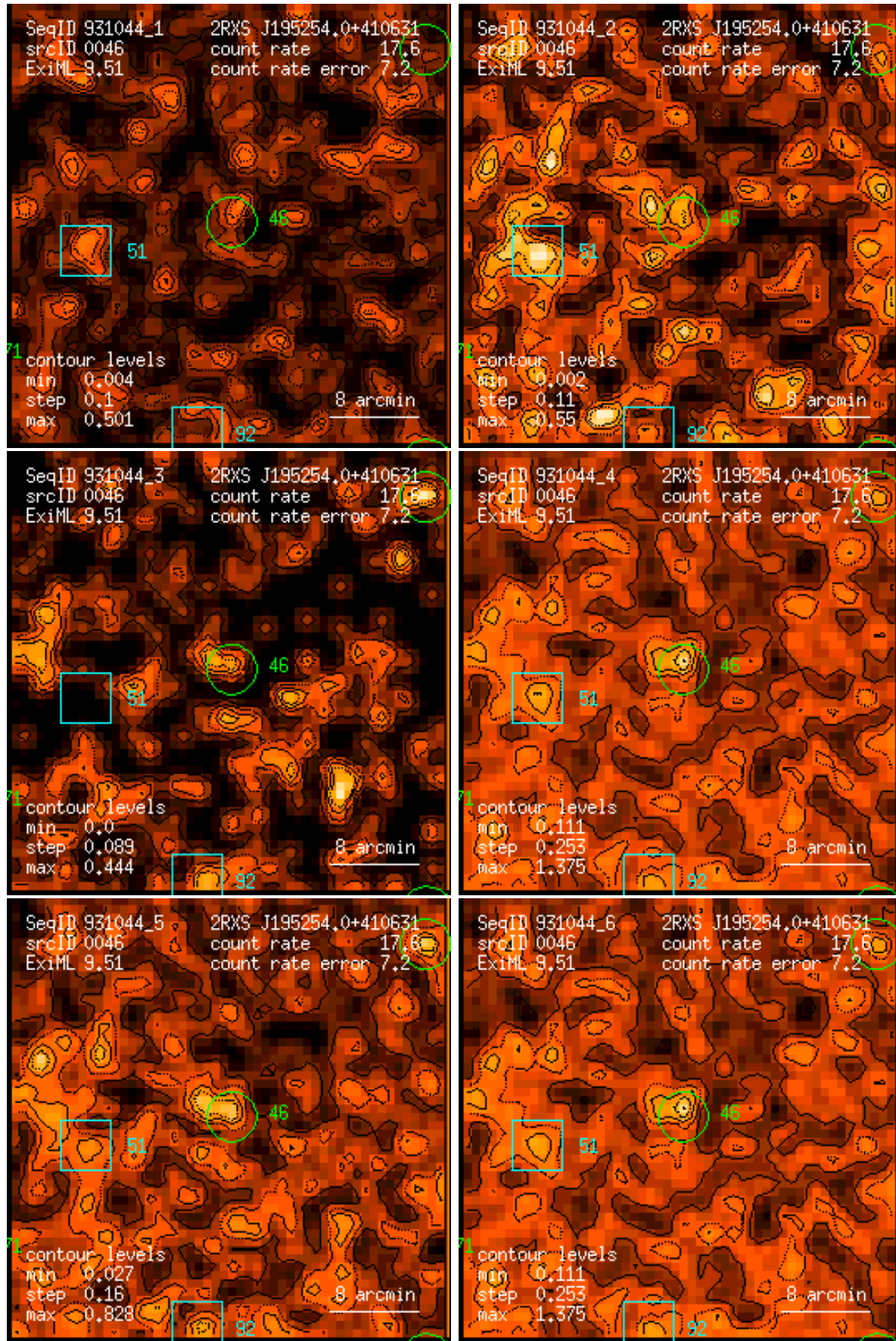
Figure 46: RASS 931044: detection 0046: band rate images, Gaussian filter: (1) PSPC channels 11 – 41, (2) 52 – 90, (3) 91 – 201, (4) 11 – 235, (5) 52 – 201, (6) 11 – 201. Broad band rates in counts/ks. Band rate contour levels in counts/ks/arcmin 2 .
