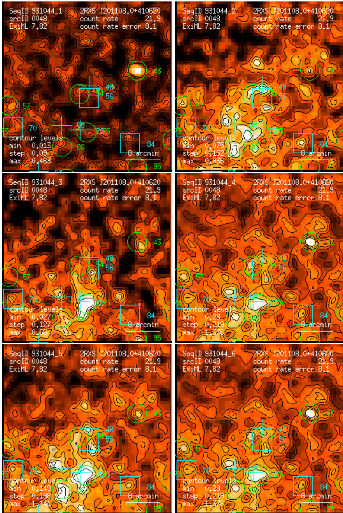
Figure 48: RASS 931044: detection 0048: band rate images, Gaussian filter: (1) PSPC channels 11 – 41, (2) 52 – 90, (3) 91 – 201, (4) 11 – 235, (5) 52 – 201, (6) 11 – 201. Broad band rates in counts/ks. Band rate contour levels in counts/ks/arcmin 2 .
