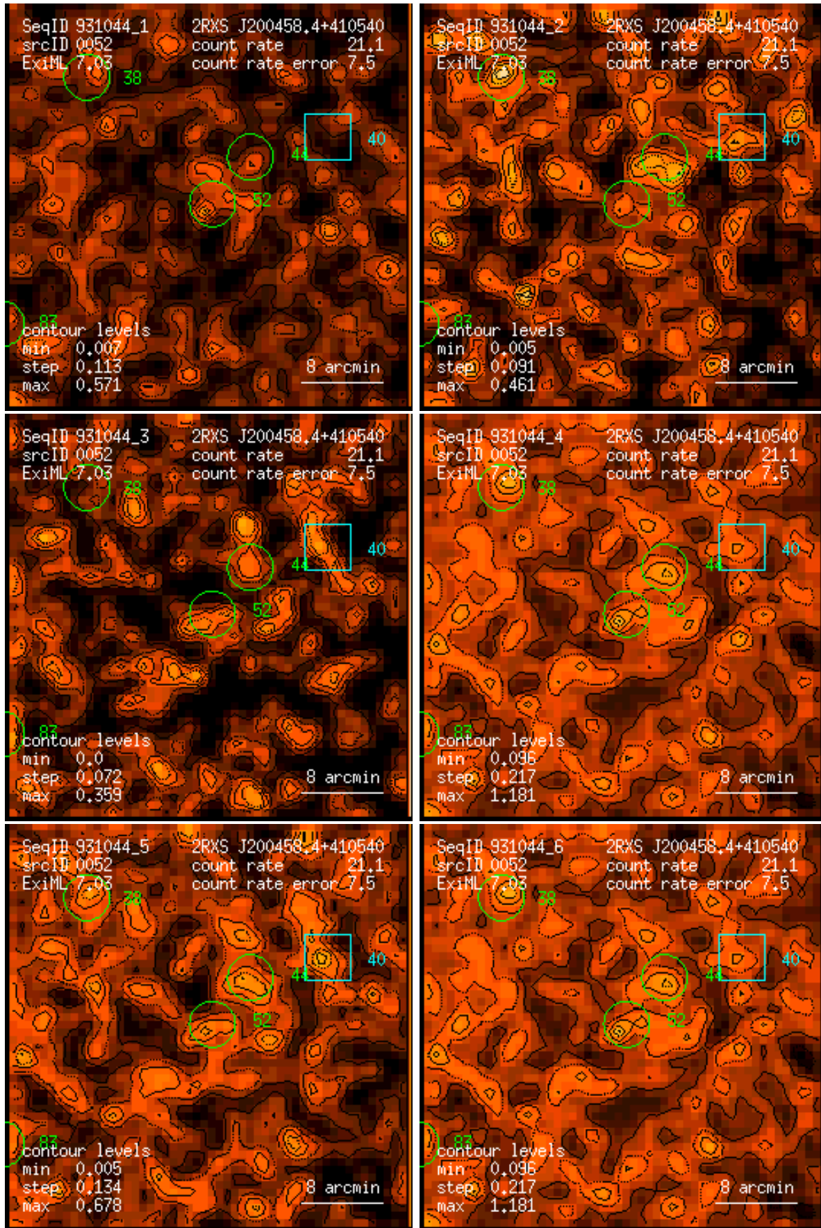
Figure 52: RASS 931044: detection 0052: band rate images, Gaussian filter: (1) PSPC channels 11 – 41, (2) 52 – 90, (3) 91 – 201, (4) 11 – 235, (5) 52 – 201, (6) 11 – 201. Broad band rates in counts/ks. Band rate contour levels in counts/ks/arcmin 2 .
