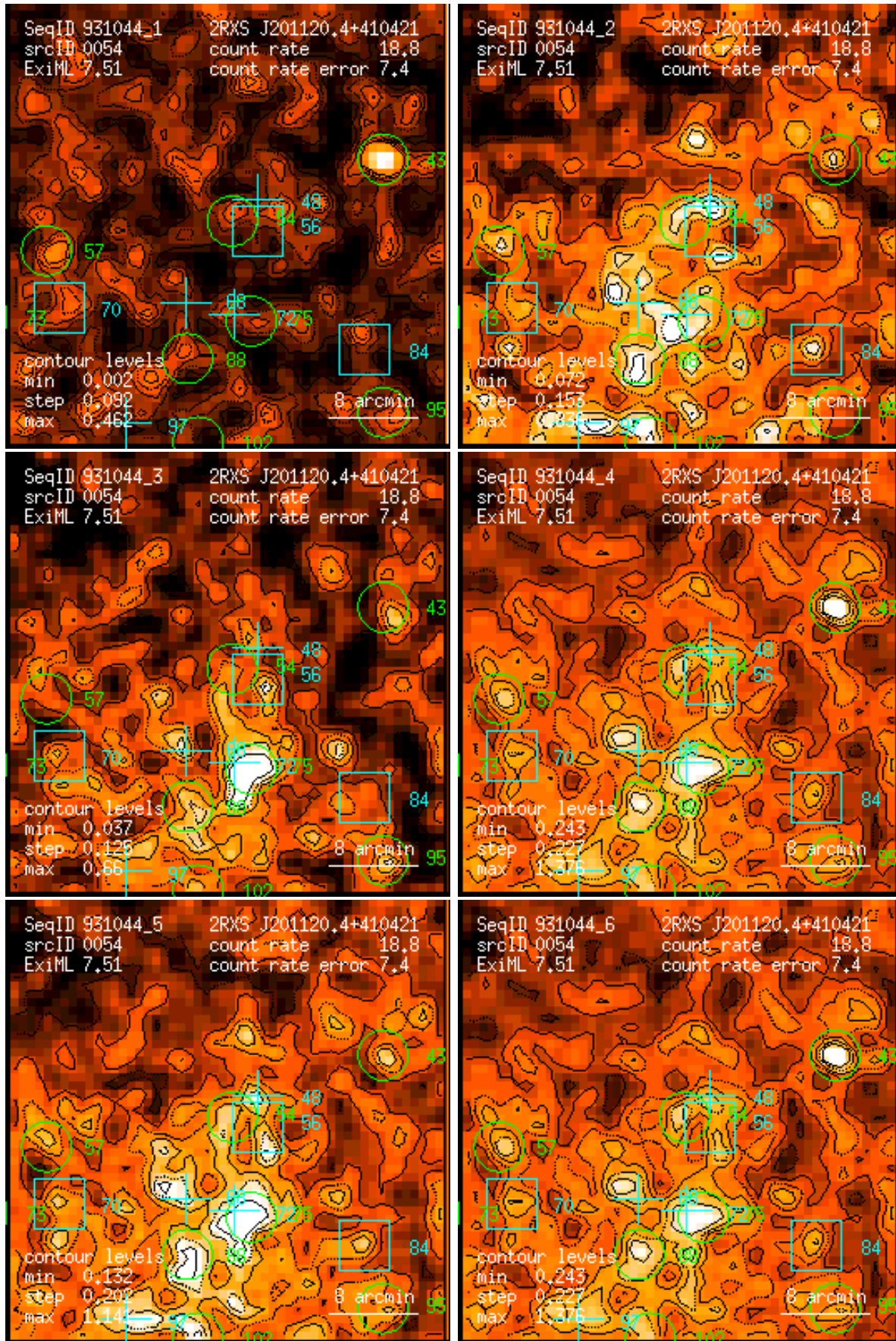
Figure 54: RASS 931044: detection 0054: band rate images, Gaussian filter: (1) PSPC channels 11 – 41, (2) 52 – 90, (3) 91 – 201, (4) 11 – 235, (5) 52 – 201, (6) 11 – 201. Broad band rates in counts/ks. Band rate contour levels in counts/ks/arcmin 2 .
