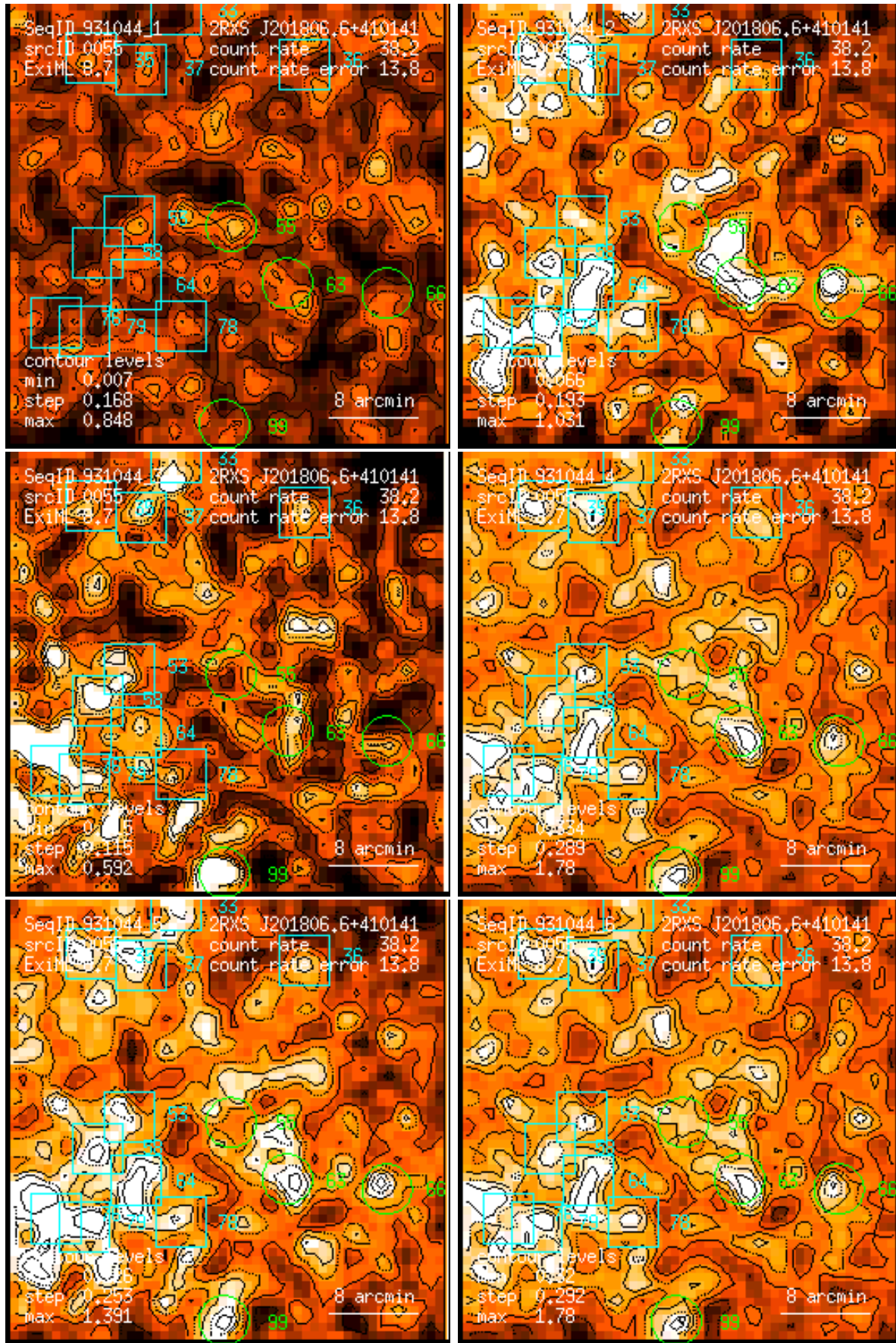
Figure 55: RASS 931044: detection 0055: band rate images, Gaussian filter: (1) PSPC channels 11 – 41, (2) 52 – 90, (3) 91 – 201, (4) 11 – 235, (5) 52 – 201, (6) 11 – 201. Broad band rates in counts/ks. Band rate contour levels in counts/ks/arcmin 2 .
