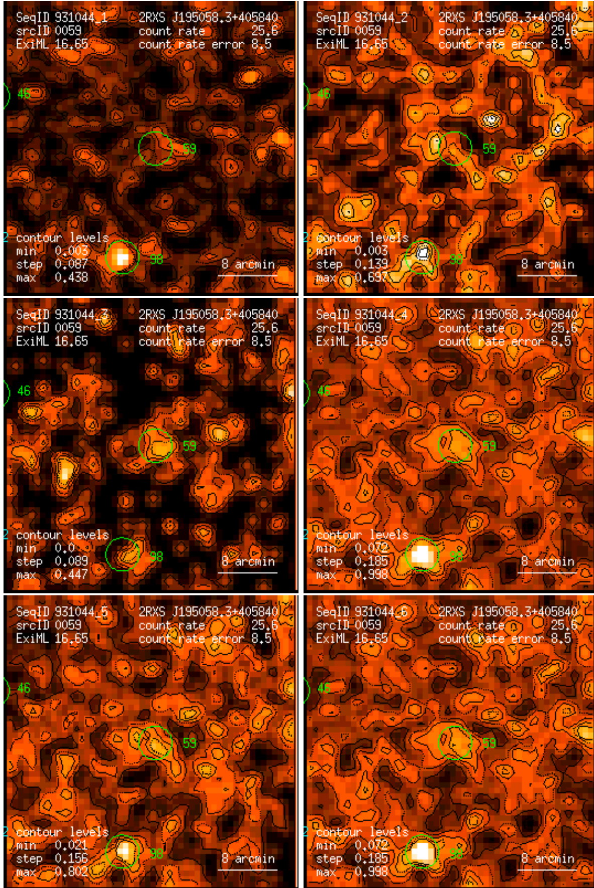
Figure 59: RASS 931044: detection 0059: band rate images, Gaussian filter: (1) PSPC channels 11 – 41, (2) 52 – 90, (3) 91 – 201, (4) 11 – 235, (5) 52 – 201, (6) 11 – 201. Broad band rates in counts/ks. Band rate contour levels in counts/ks/arcmin 2 .
