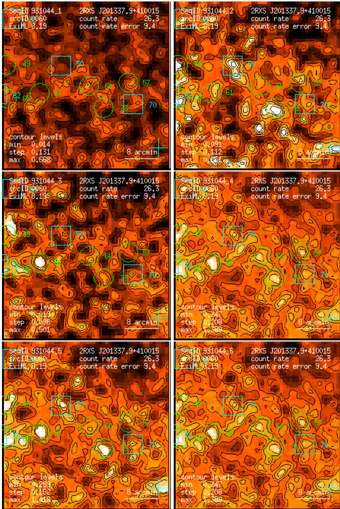
Figure 60: RASS 931044: detection 0060: band rate images, Gaussian filter: (1) PSPC channels 11 – 41, (2) 52 – 90, (3) 91 – 201, (4) 11 – 235, (5) 52 – 201, (6) 11 – 201. Broad band rates in counts/ks. Band rate contour levels in counts/ks/arcmin 2 .
