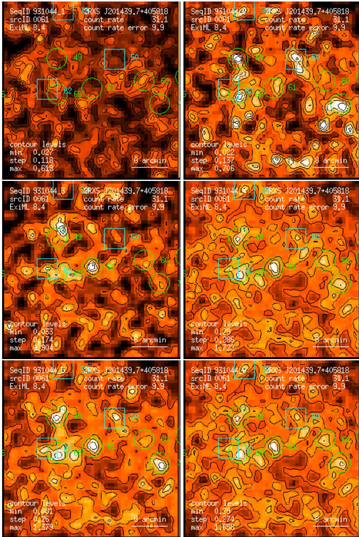
Figure 61: RASS 931044: detection 0061: band rate images, Gaussian filter: (1) PSPC channels 11 – 41, (2) 52 – 90, (3) 91 – 201, (4) 11 – 235, (5) 52 – 201, (6) 11 – 201. Broad band rates in counts/ks. Band rate contour levels in counts/ks/arcmin 2 .
