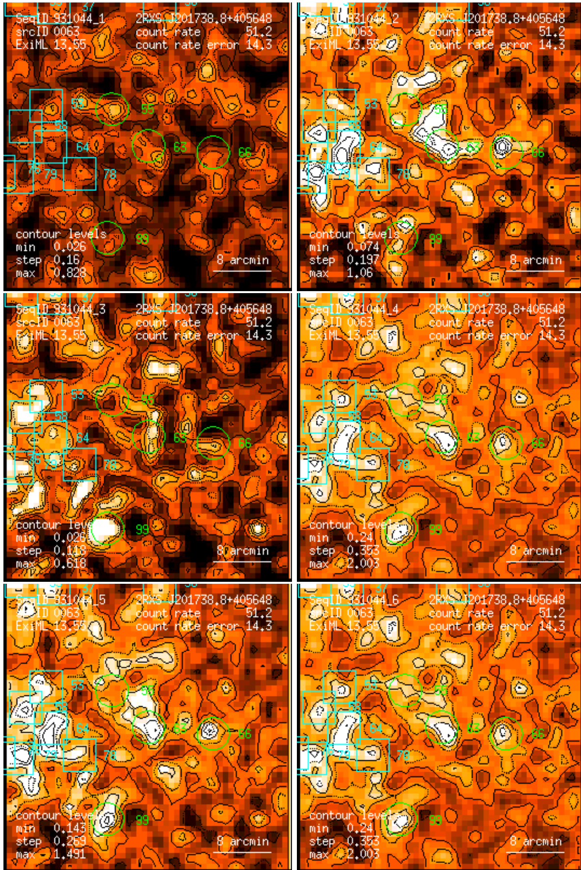
Figure 63: RASS 931044: detection 0063: band rate images, Gaussian filter: (1) PSPC channels 11 – 41, (2) 52 – 90, (3) 91 – 201, (4) 11 – 235, (5) 52 – 201, (6) 11 – 201. Broad band rates in counts/ks. Band rate contour levels in counts/ks/arcmin 2 .
