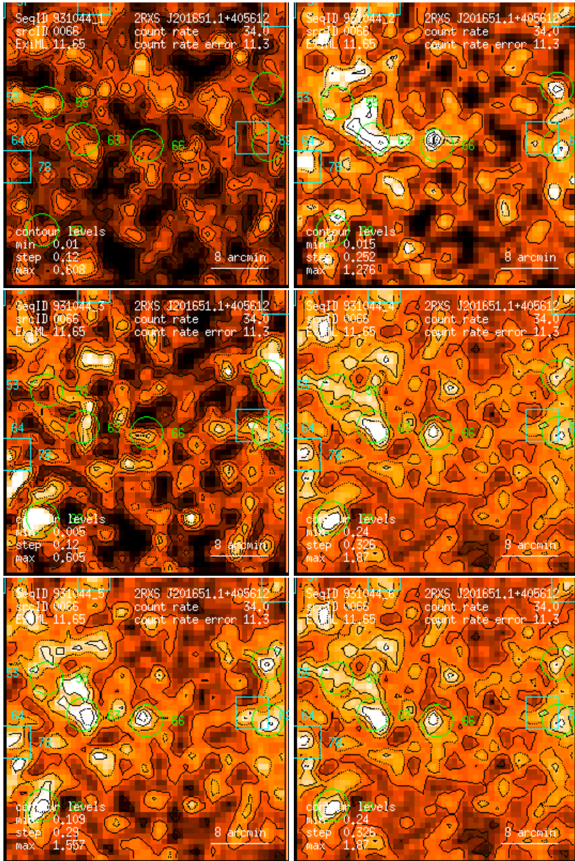
Figure 66: RASS 931044: detection 0066: band rate images, Gaussian filter: (1) PSPC channels 11 – 41, (2) 52 – 90, (3) 91 – 201, (4) 11 – 235, (5) 52 – 201, (6) 11 – 201. Broad band rates in counts/ks. Band rate contour levels in counts/ks/arcmin 2 .
