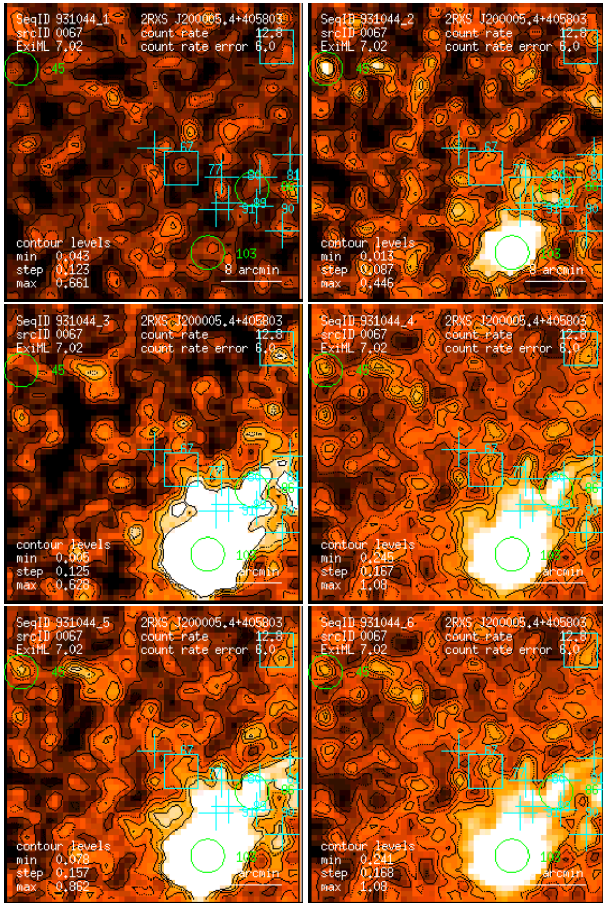
Figure 67: RASS 931044: detection 0067: band rate images, Gaussian filter: (1) PSPC channels 11 – 41, (2) 52 – 90, (3) 91 – 201, (4) 11 – 235, (5) 52 – 201, (6) 11 – 201. Broad band rates in counts/ks. Band rate contour levels in counts/ks/arcmin 2 .
