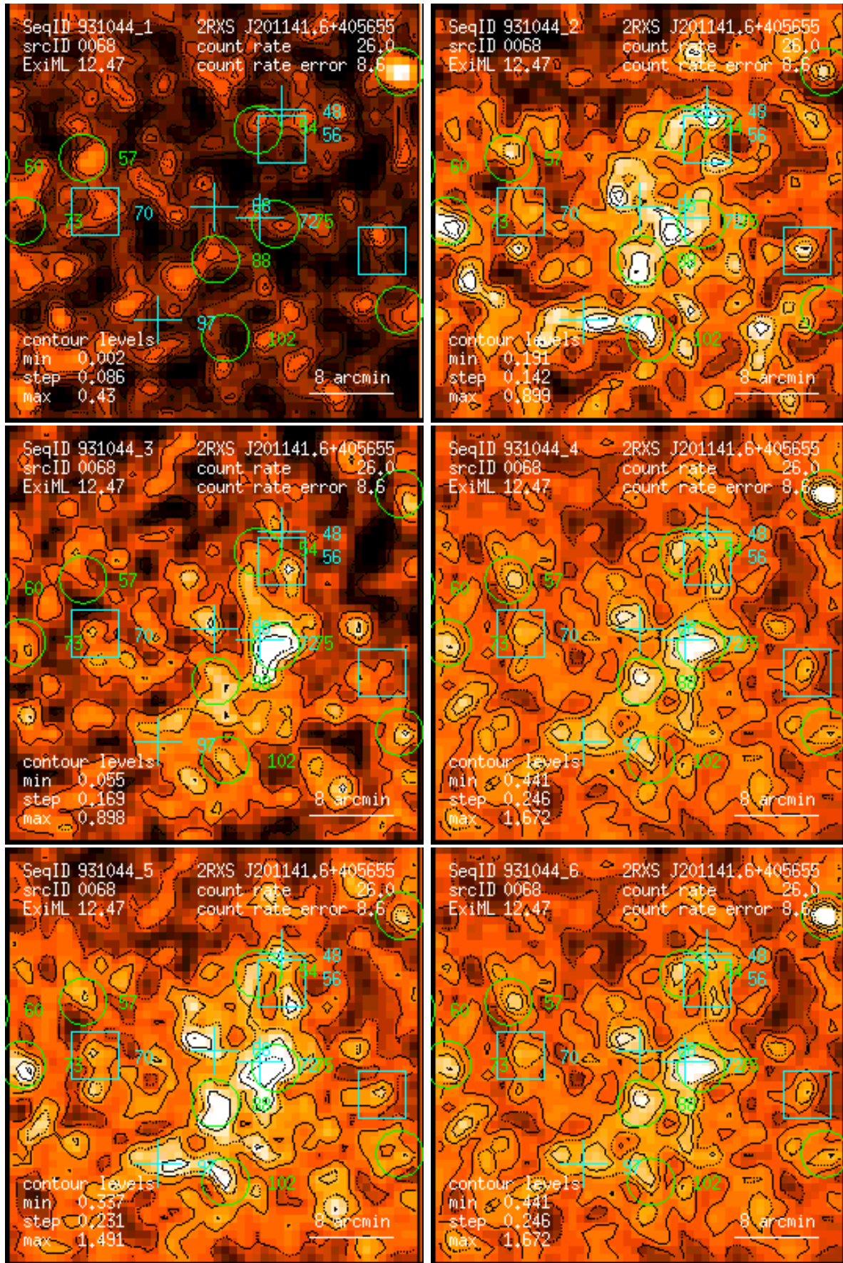
Figure 68: RASS 931044: detection 0068: band rate images, Gaussian filter: (1) PSPC channels 11 – 41, (2) 52 – 90, (3) 91 – 201, (4) 11 – 235, (5) 52 – 201, (6) 11 – 201. Broad band rates in counts/ks. Band rate contour levels in counts/ks/arcmin 2 .
