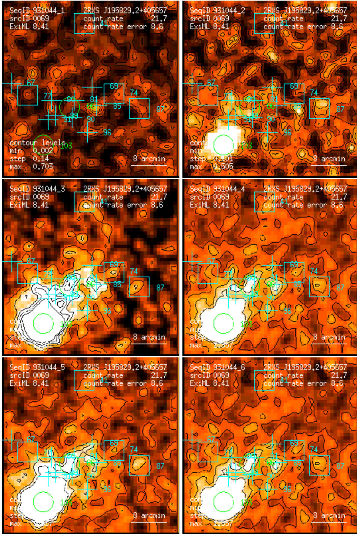
Figure 69: RASS 931044: detection 0069: band rate images, Gaussian filter: (1) PSPC channels 11 – 41, (2) 52 – 90, (3) 91 – 201, (4) 11 – 235, (5) 52 – 201, (6) 11 – 201. Broad band rates in counts/ks. Band rate contour levels in counts/ks/arcmin 2 .
