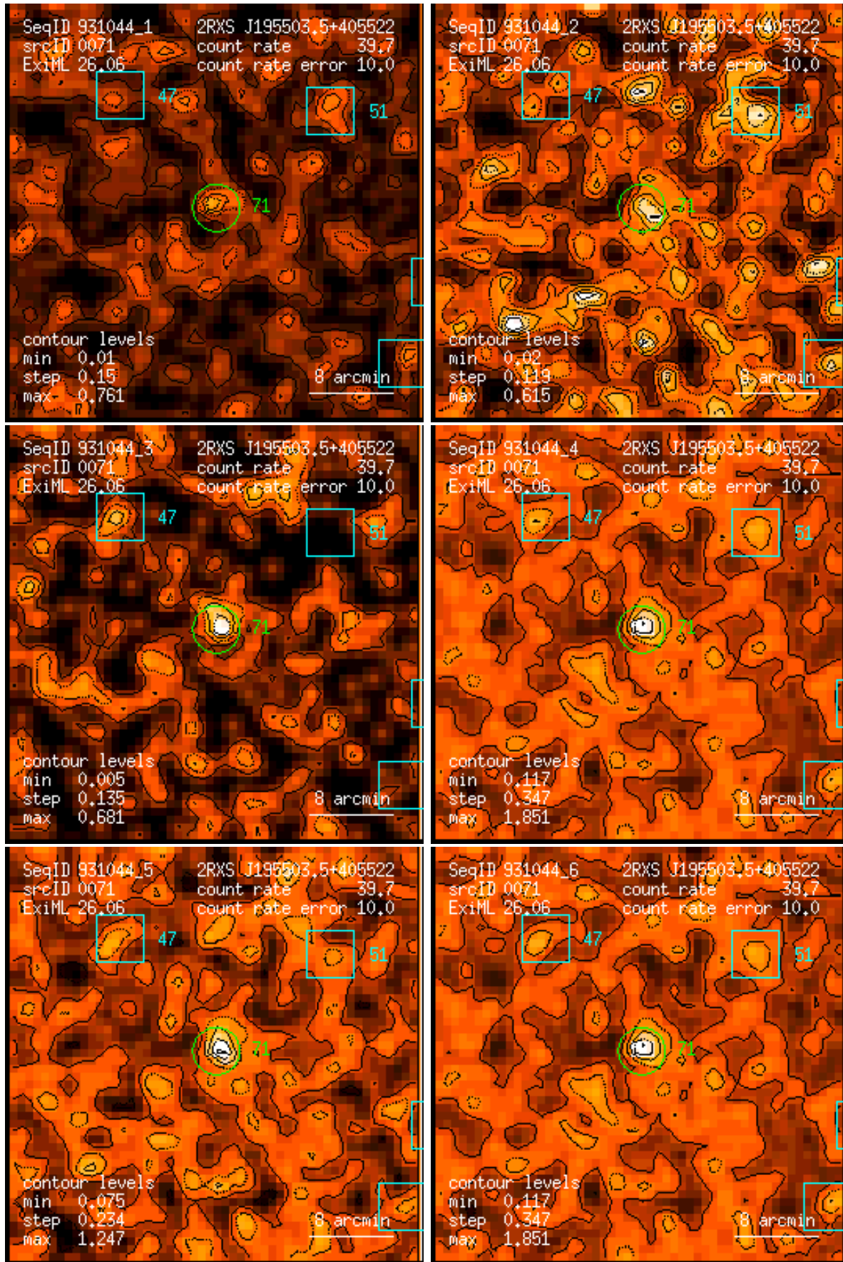
Figure 71: RASS 931044: detection 0071: band rate images, Gaussian filter: (1) PSPC channels 11 – 41, (2) 52 – 90, (3) 91 – 201, (4) 11 – 235, (5) 52 – 201, (6) 11 – 201. Broad band rates in counts/ks. Band rate contour levels in counts/ks/arcmin 2 .
