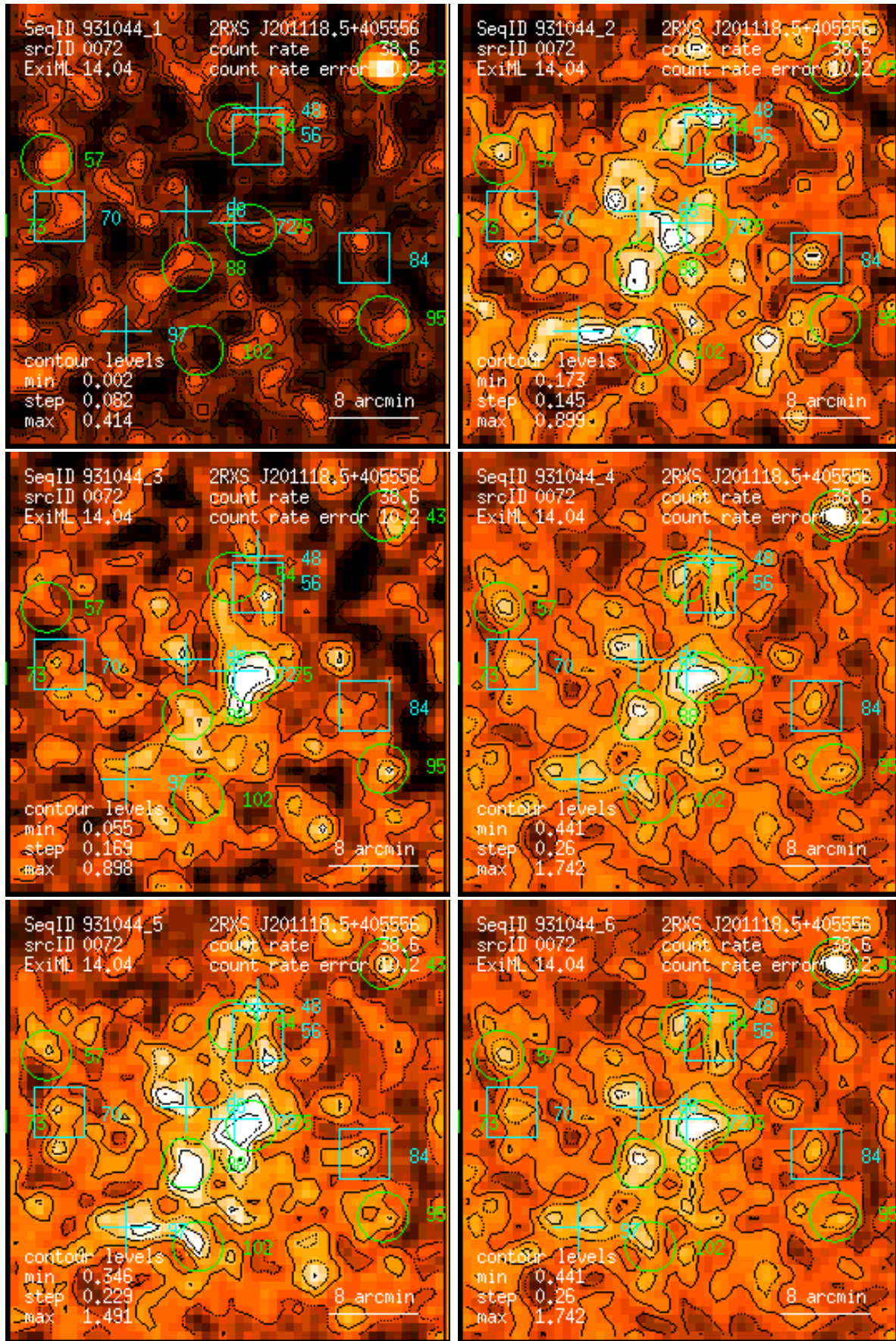
Figure 72: RASS 931044: detection 0072: band rate images, Gaussian filter: (1) PSPC channels 11 – 41, (2) 52 – 90, (3) 91 – 201, (4) 11 – 235, (5) 52 – 201, (6) 11 – 201. Broad band rates in counts/ks. Band rate contour levels in counts/ks/arcmin 2 .
