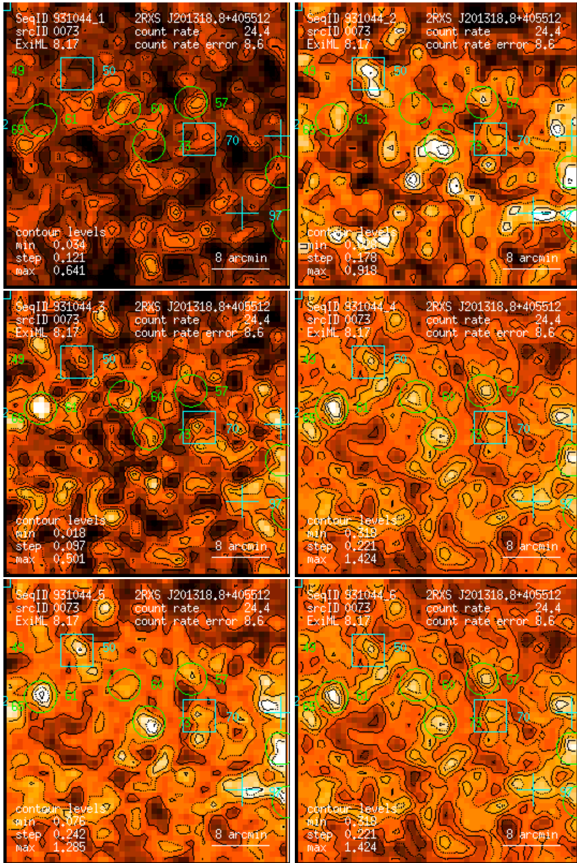
Figure 73: RASS 931044: detection 0073: band rate images, Gaussian filter: (1) PSPC channels 11 – 41, (2) 52 – 90, (3) 91 – 201, (4) 11 – 235, (5) 52 – 201, (6) 11 – 201. Broad band rates in counts/ks. Band rate contour levels in counts/ks/arcmin 2 .
