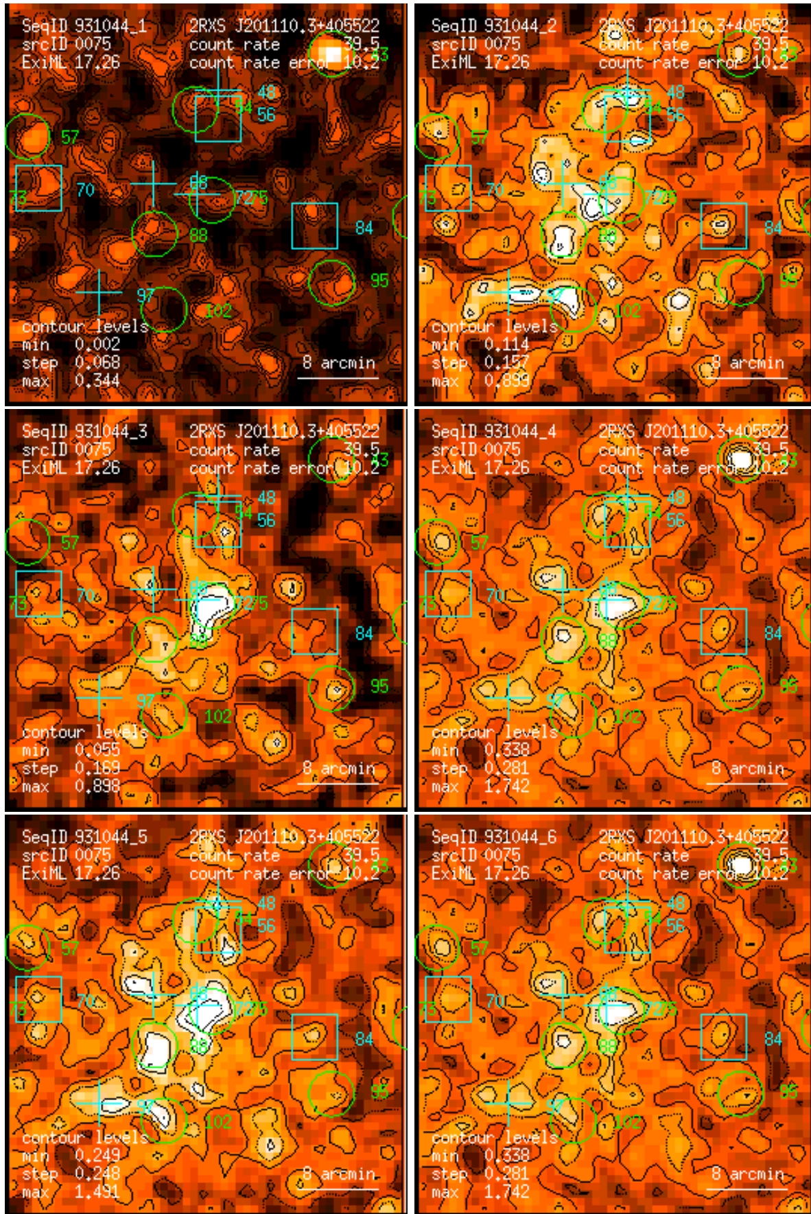
Figure 75: RASS 931044: detection 0075: band rate images, Gaussian filter: (1) PSPC channels 11 – 41, (2) 52 – 90, (3) 91 – 201, (4) 11 – 235, (5) 52 – 201, (6) 11 – 201. Broad band rates in counts/ks. Band rate contour levels in counts/ks/arcmin 2 .
