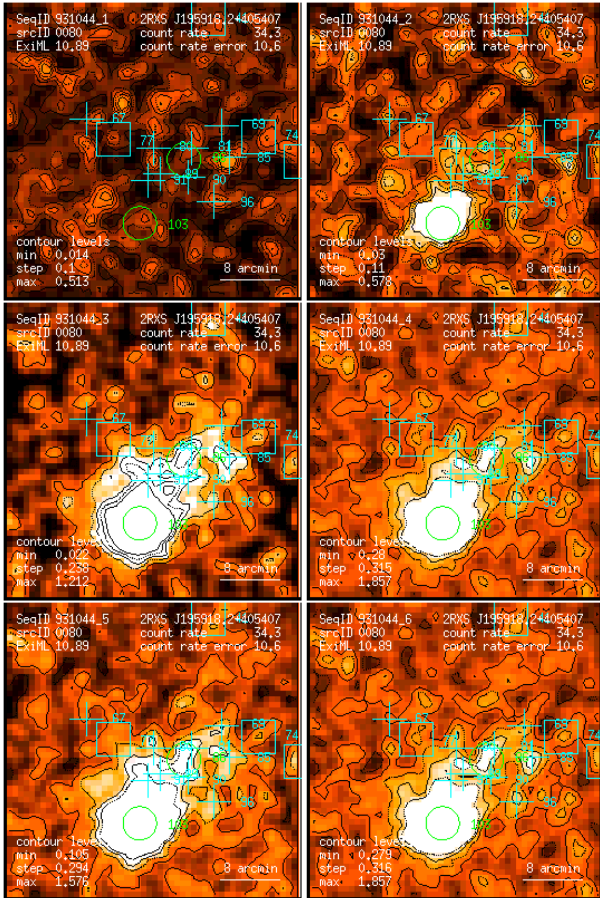
Figure 80: RASS 931044: detection 0080: band rate images, Gaussian filter: (1) PSPC channels 11 – 41, (2) 52 – 90, (3) 91 – 201, (4) 11 – 235, (5) 52 – 201, (6) 11 – 201. Broad band rates in counts/ks. Band rate contour levels in counts/ks/arcmin 2 .
