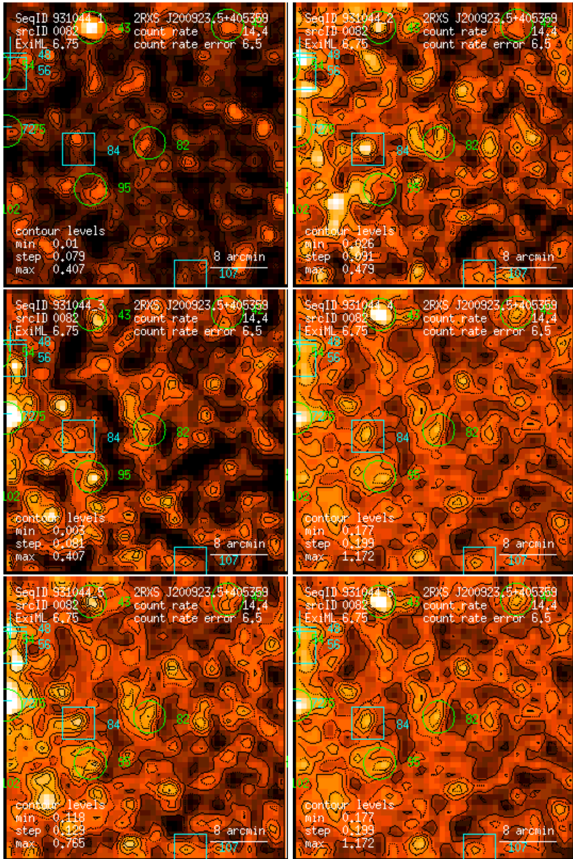
Figure 82: RASS 931044: detection 0082: band rate images, Gaussian filter: (1) PSPC channels 11 – 41, (2) 52 – 90, (3) 91 – 201, (4) 11 – 235, (5) 52 – 201, (6) 11 – 201. Broad band rates in counts/ks. Band rate contour levels in counts/ks/arcmin 2 .
