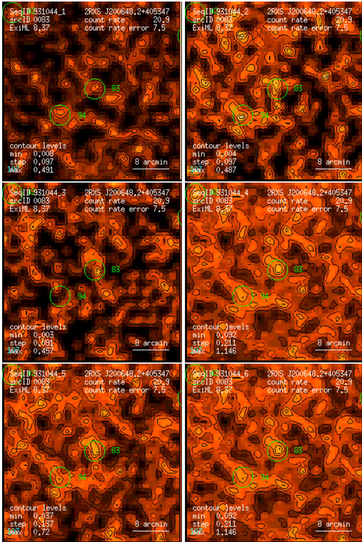
Figure 83: RASS 931044: detection 0083: band rate images, Gaussian filter: (1) PSPC channels 11 – 41, (2) 52 – 90, (3) 91 – 201, (4) 11 – 235, (5) 52 – 201, (6) 11 – 201. Broad band rates in counts/ks. Band rate contour levels in counts/ks/arcmin 2 .
