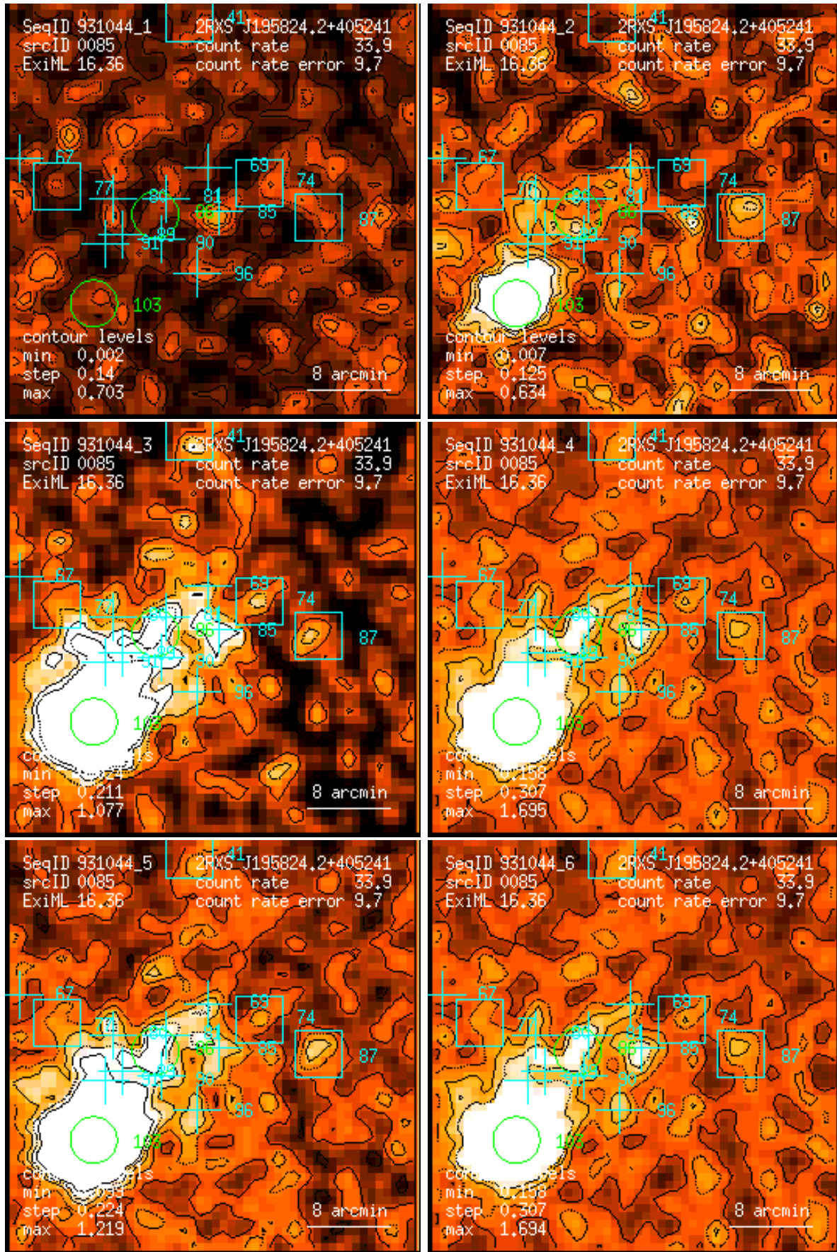
Figure 85: RASS 931044: detection 0085: band rate images, Gaussian filter: (1) PSPC channels 11 – 41, (2) 52 – 90, (3) 91 – 201, (4) 11 – 235, (5) 52 – 201, (6) 11 – 201. Broad band rates in counts/ks. Band rate contour levels in counts/ks/arcmin 2 .
