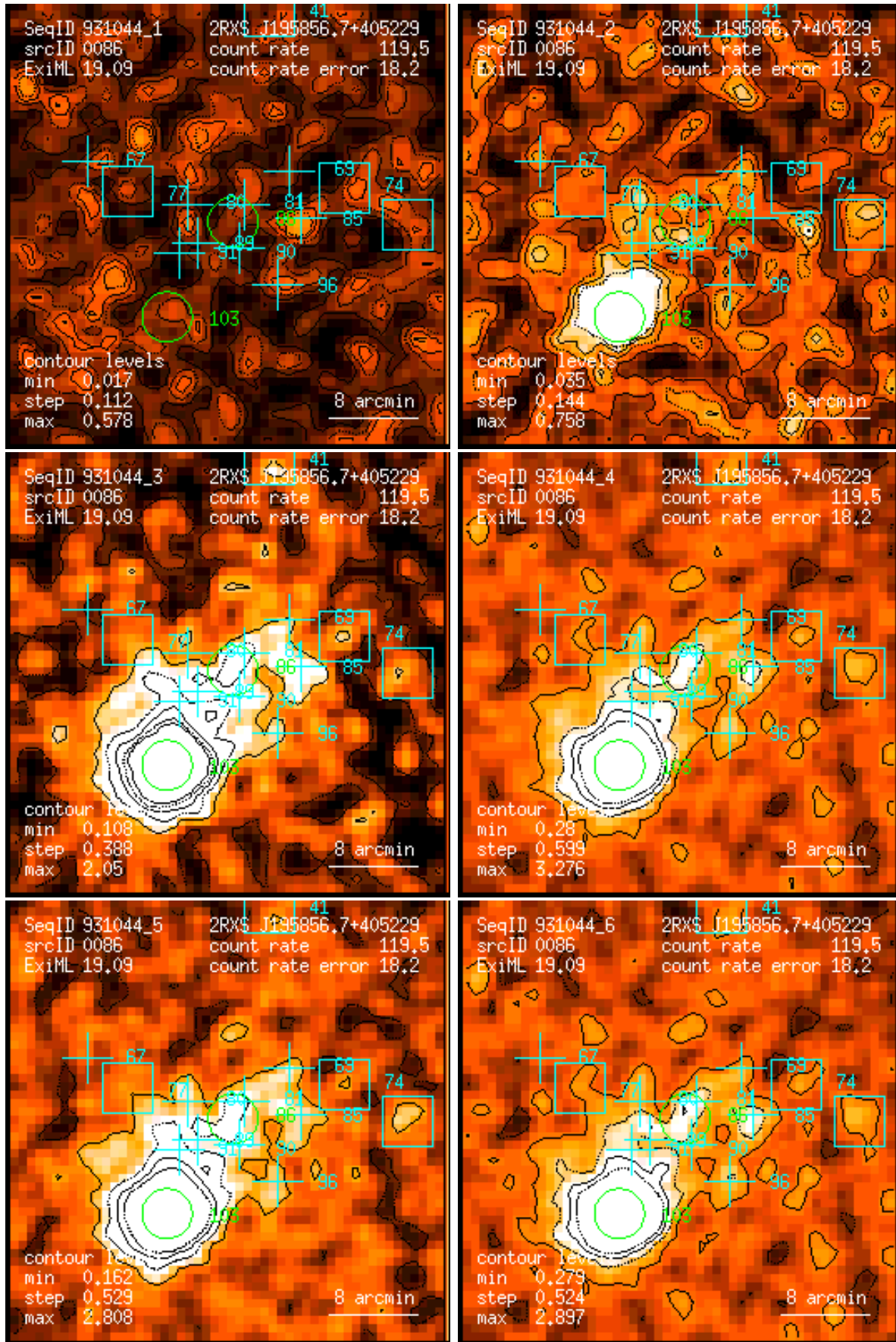
Figure 86: RASS 931044: detection 0086: band rate images, Gaussian filter: (1) PSPC channels 11 – 41, (2) 52 – 90, (3) 91 – 201, (4) 11 – 235, (5) 52 – 201, (6) 11 – 201. Broad band rates in counts/ks. Band rate contour levels in counts/ks/arcmin 2 .
