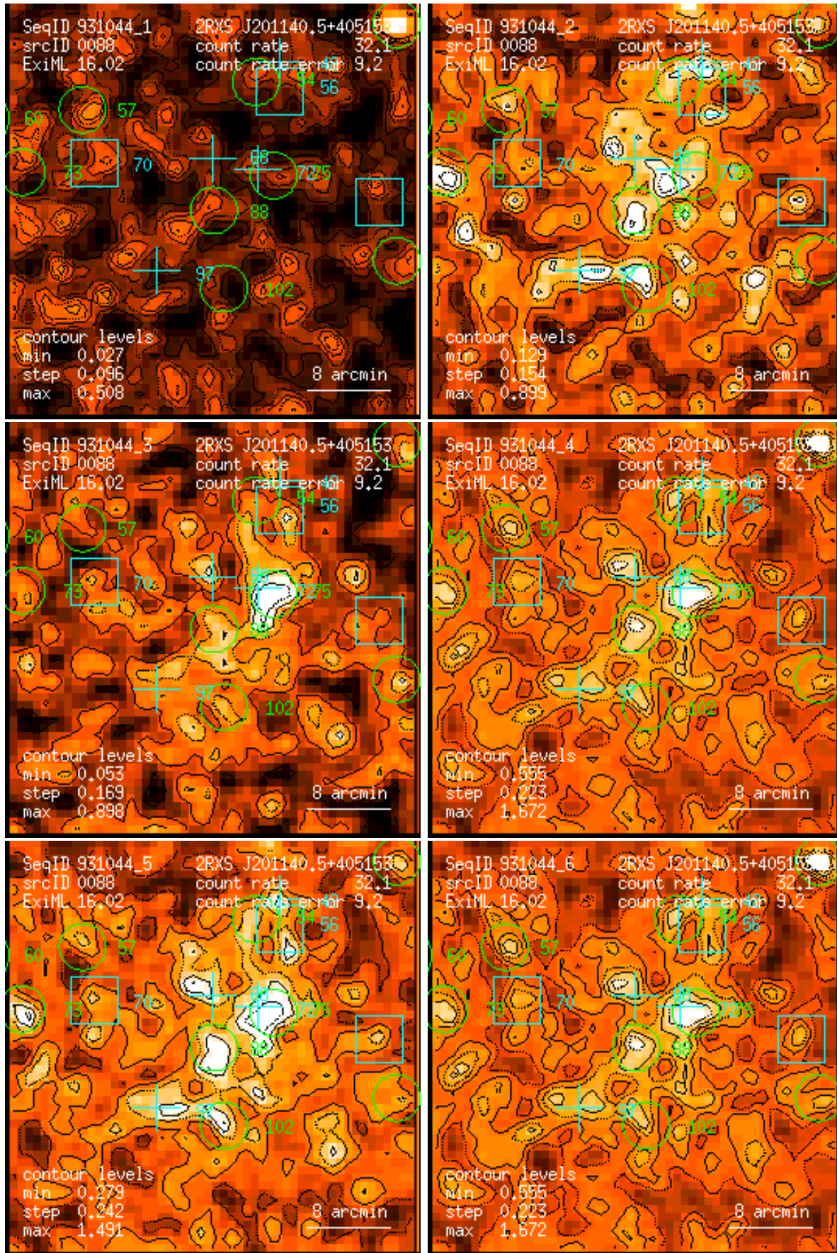
Figure 88: RASS 931044: detection 0088: band rate images, Gaussian filter: (1) PSPC channels 11 – 41, (2) 52 – 90, (3) 91 – 201, (4) 11 – 235, (5) 52 – 201, (6) 11 – 201. Broad band rates in counts/ks. Band rate contour levels in counts/ks/arcmin 2 .
