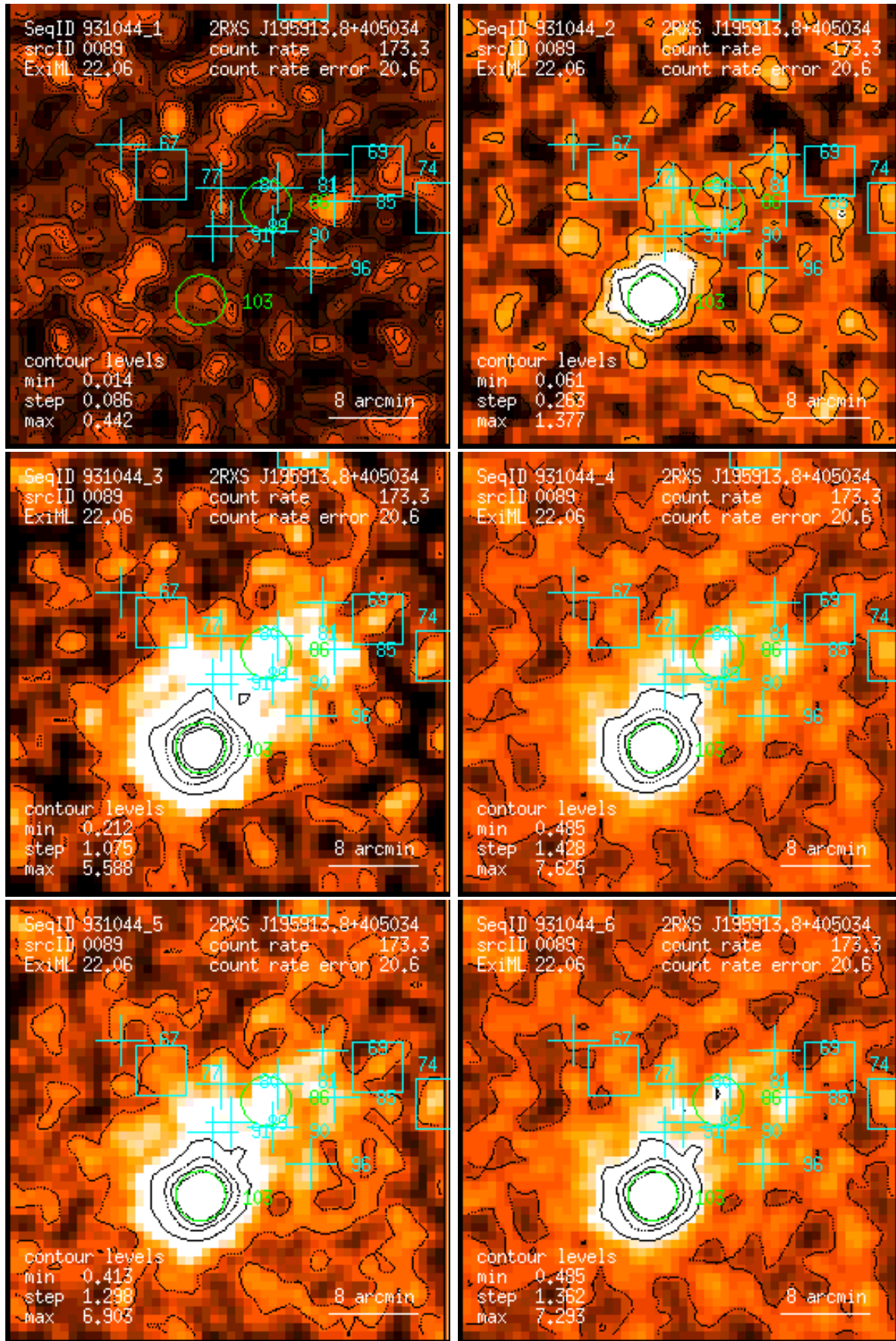
Figure 89: RASS 931044: detection 0089: band rate images, Gaussian filter: (1) PSPC channels 11 – 41, (2) 52 – 90, (3) 91 – 201, (4) 11 – 235, (5) 52 – 201, (6) 11 – 201. Broad band rates in counts/ks. Band rate contour levels in counts/ks/arcmin 2 .
