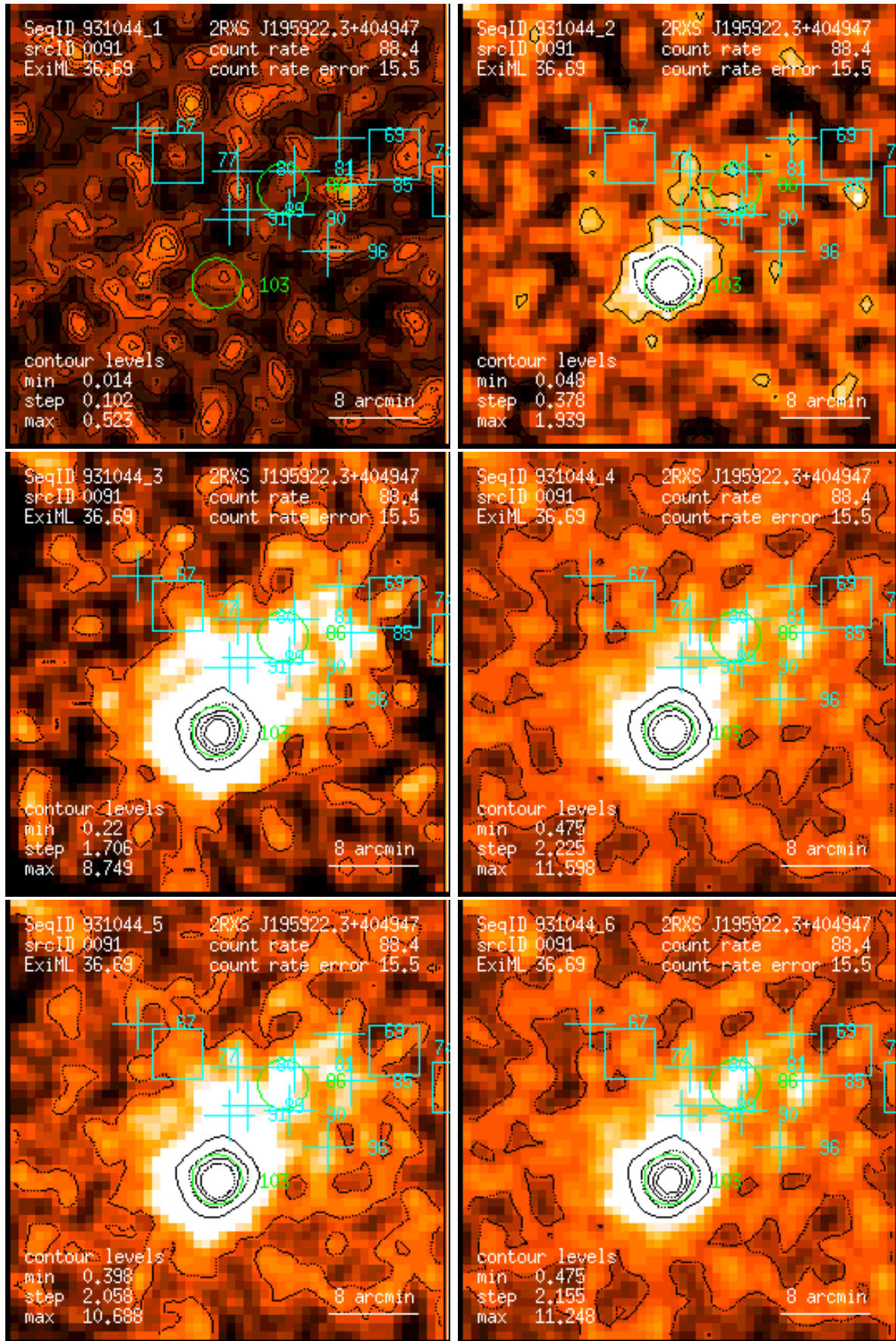
Figure 91: RASS 931044: detection 0091: band rate images, Gaussian filter: (1) PSPC channels 11 – 41, (2) 52 – 90, (3) 91 – 201, (4) 11 – 235, (5) 52 – 201, (6) 11 – 201. Broad band rates in counts/ks. Band rate contour levels in counts/ks/arcmin 2 .
