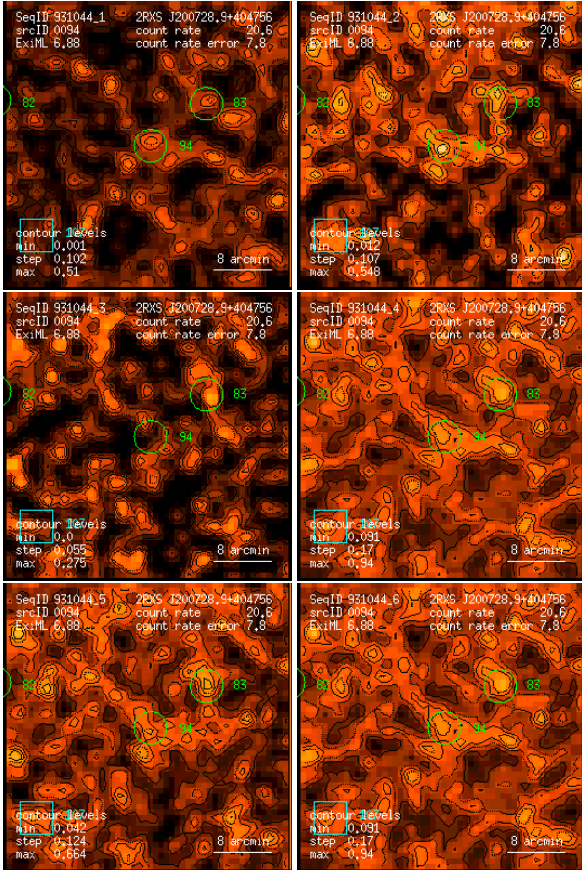
Figure 94: RASS 931044: detection 0094: band rate images, Gaussian filter: (1) PSPC channels 11 – 41, (2) 52 – 90, (3) 91 – 201, (4) 11 – 235, (5) 52 – 201, (6) 11 – 201. Broad band rates in counts/ks. Band rate contour levels in counts/ks/arcmin 2 .
