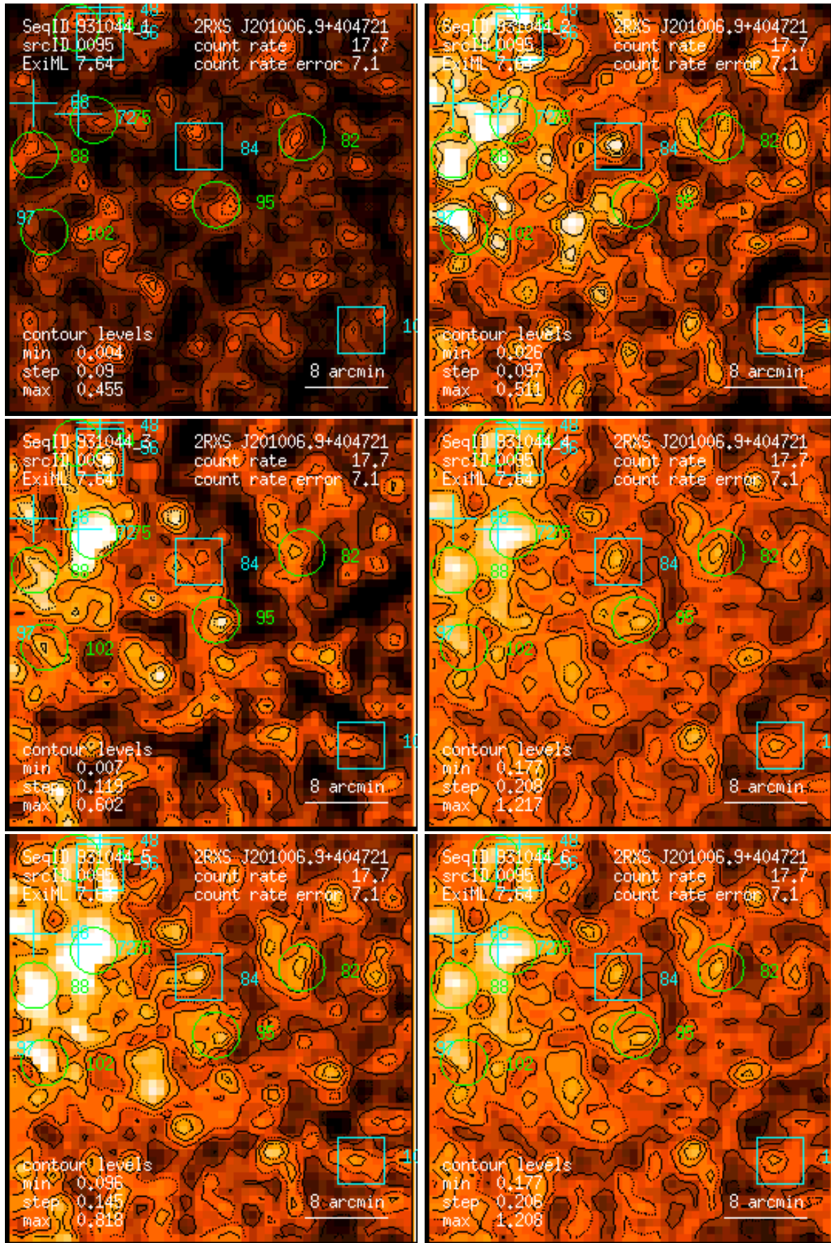
Figure 95: RASS 931044: detection 0095: band rate images, Gaussian filter: (1) PSPC channels 11 – 41, (2) 52 – 90, (3) 91 – 201, (4) 11 – 235, (5) 52 – 201, (6) 11 – 201. Broad band rates in counts/ks. Band rate contour levels in counts/ks/arcmin 2 .
