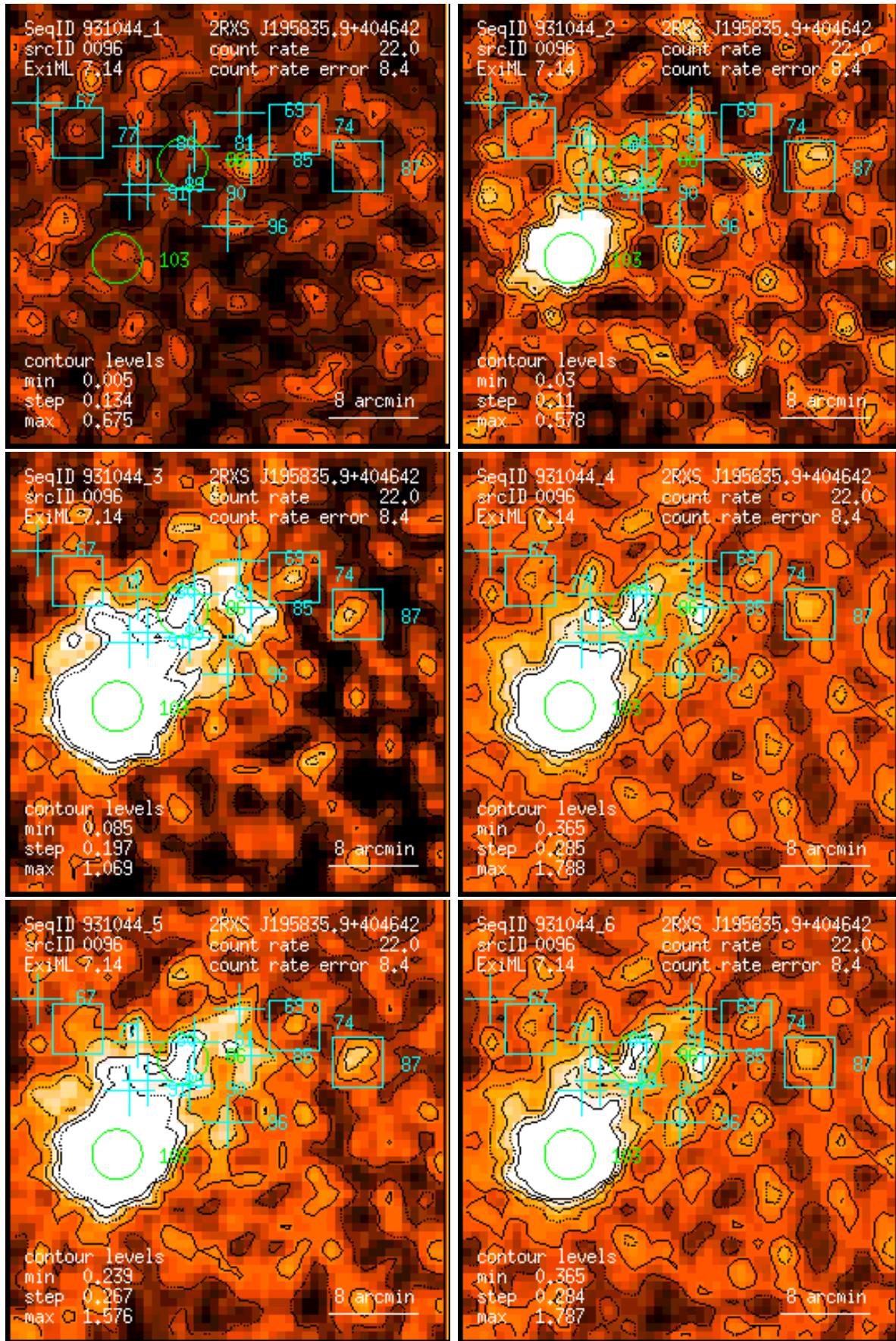
Figure 96: RASS 931044: detection 0096: band rate images, Gaussian filter: (1) PSPC channels 11 – 41, (2) 52 – 90, (3) 91 – 201, (4) 11 – 235, (5) 52 – 201, (6) 11 – 201. Broad band rates in counts/ks. Band rate contour levels in counts/ks/arcmin 2 .
