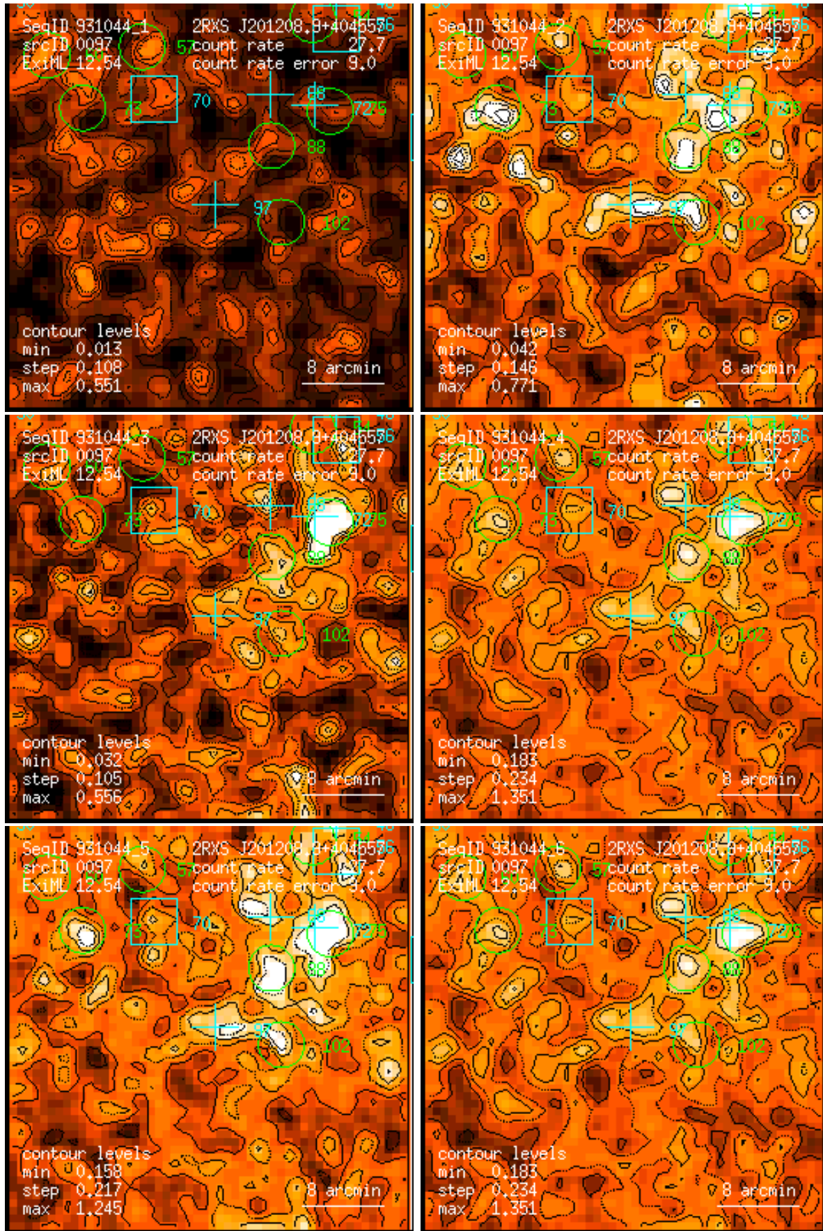
Figure 97: RASS 931044: detection 0097: band rate images, Gaussian filter: (1) PSPC channels 11 – 41, (2) 52 – 90, (3) 91 – 201, (4) 11 – 235, (5) 52 – 201, (6) 11 – 201. Broad band rates in counts/ks. Band rate contour levels in counts/ks/arcmin 2 .
