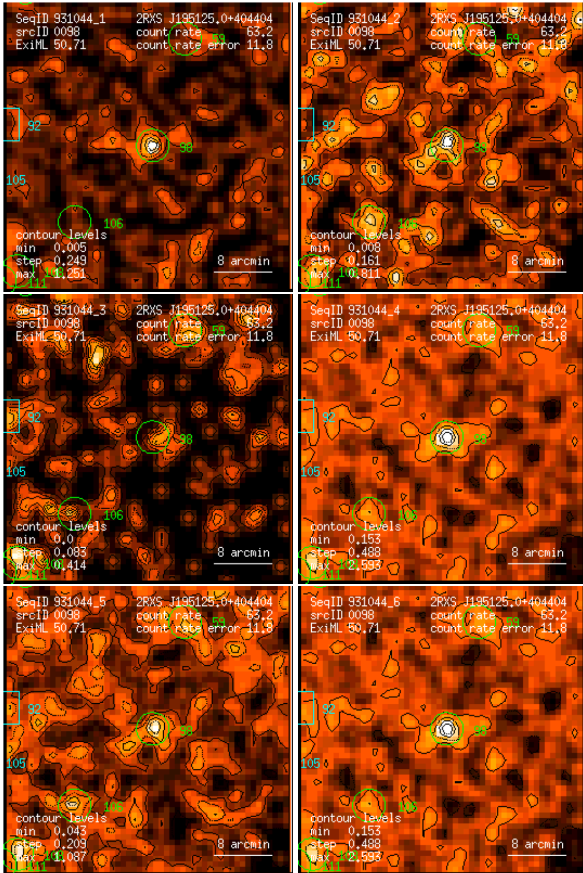
Figure 98: RASS 931044: detection 0098: band rate images, Gaussian filter: (1) PSPC channels 11 – 41, (2) 52 – 90, (3) 91 – 201, (4) 11 – 235, (5) 52 – 201, (6) 11 – 201. Broad band rates in counts/ks. Band rate contour levels in counts/ks/arcmin 2 .
