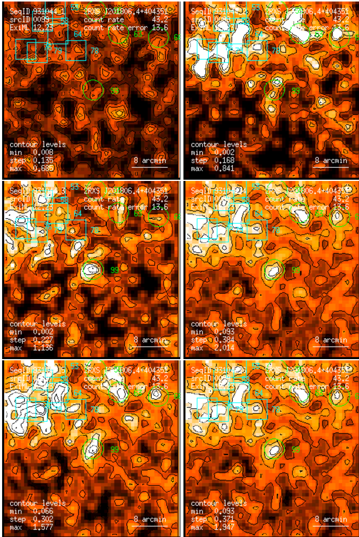
Figure 99: RASS 931044: detection 0099: band rate images, Gaussian filter: (1) PSPC channels 11 – 41, (2) 52 – 90, (3) 91 – 201, (4) 11 – 235, (5) 52 – 201, (6) 11 – 201. Broad band rates in counts/ks. Band rate contour levels in counts/ks/arcmin 2 .
